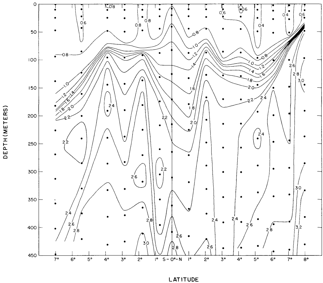
Fig. 17. -- Inorganic phosphate . Northbound section along 140^{\circ}\text{W} . longitude, 7^{\circ}\text{S} . to 8^{\circ}\text{N} ., stations 17-31, June 3-8, 1952. Phosphate in microgram atoms per liter, isopleth interval 0.2 \mu\text{g at/l} .
