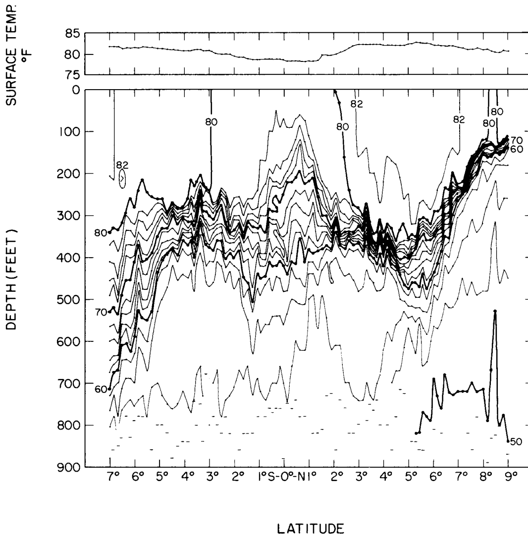
Fig. 6. -- Surface temperatures and vertical temperature section. Northbound; stations 45-60, June 14-20, 1952. Upper panel. Surface temperatures as read at each bathythermograph lowering. Lower panel. Temperature section based on bathythermograph lowerings, isotherms at 2°F. interval, depth of lowering shown by small, horizontal dashed line.
