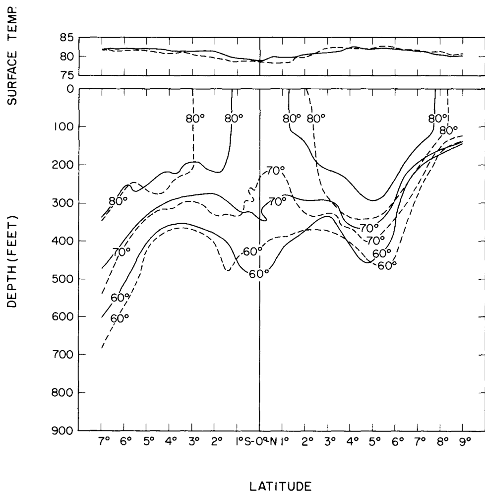
Fig. 28. -- Upper panel. Surface temperatures, first leg (solid curves) and fourth leg (broken curve) of Hugh M. Smith cruise 15. Lower panel. Smoothed (by inspection) 60^{\circ} , 70^{\circ} , and 80^{\circ} isotherms for the first leg (stations 1-17, May 28 - June 3, 1952, solid curves) and fourth leg (stations 45-60, June 14-20, 1952, broken curves) of Hugh M. Smith cruise 15.
