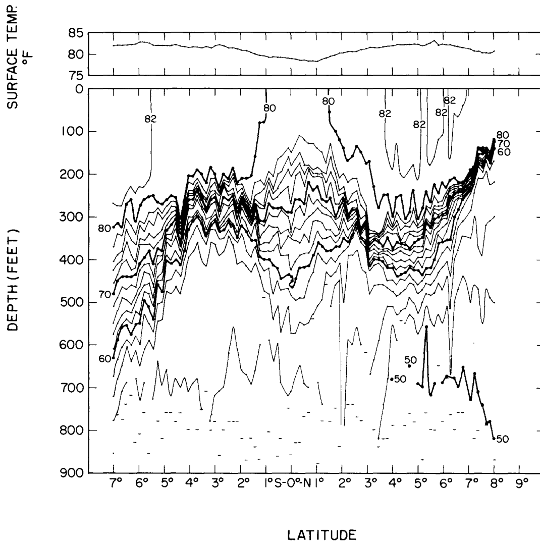
Fig. 4. -- Surface temperatures and vertical temperature section. Northbound, stations 17-31, June 3-8, 1952. Upper panel. Surface temperatures as read at each bathythermograph lowering. Lower panel. Temperature section based on bathythermograph lowerings, isotherms at 2°F. interval, depth of lowering shown by small, horizontal dashed line.
