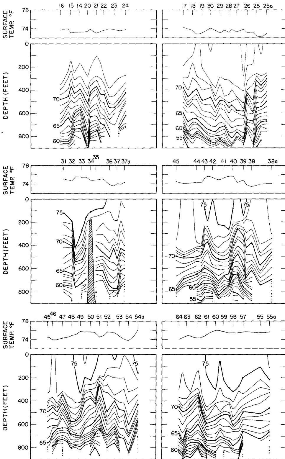
Figure 24. -- Vertical bathythermograph temperature ( ^{\circ} F.) sections from stations 24 to 16, 25a to 17, 37a to 31, 38a to 45, 54a to 45, and 55a to 64, H. M. Smith cruise 20, March 1953. The upper panels show the surface bucket temperatures in F.
