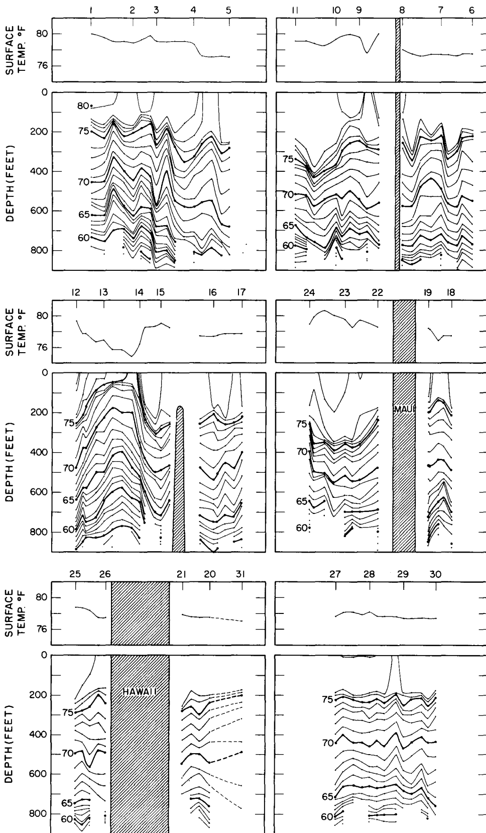
Figure 10. -- Vertical bathythermograph temperature ( ^{\circ} F.) sections from stations 5 to 1, 6 to 11, 17 to 12, 18 to 24, 31 to 25, and 30 to 27, H. M. Smith cruise 17, September 1952. The upper panels show the surface bucket temperatures in ^{\circ} F.
