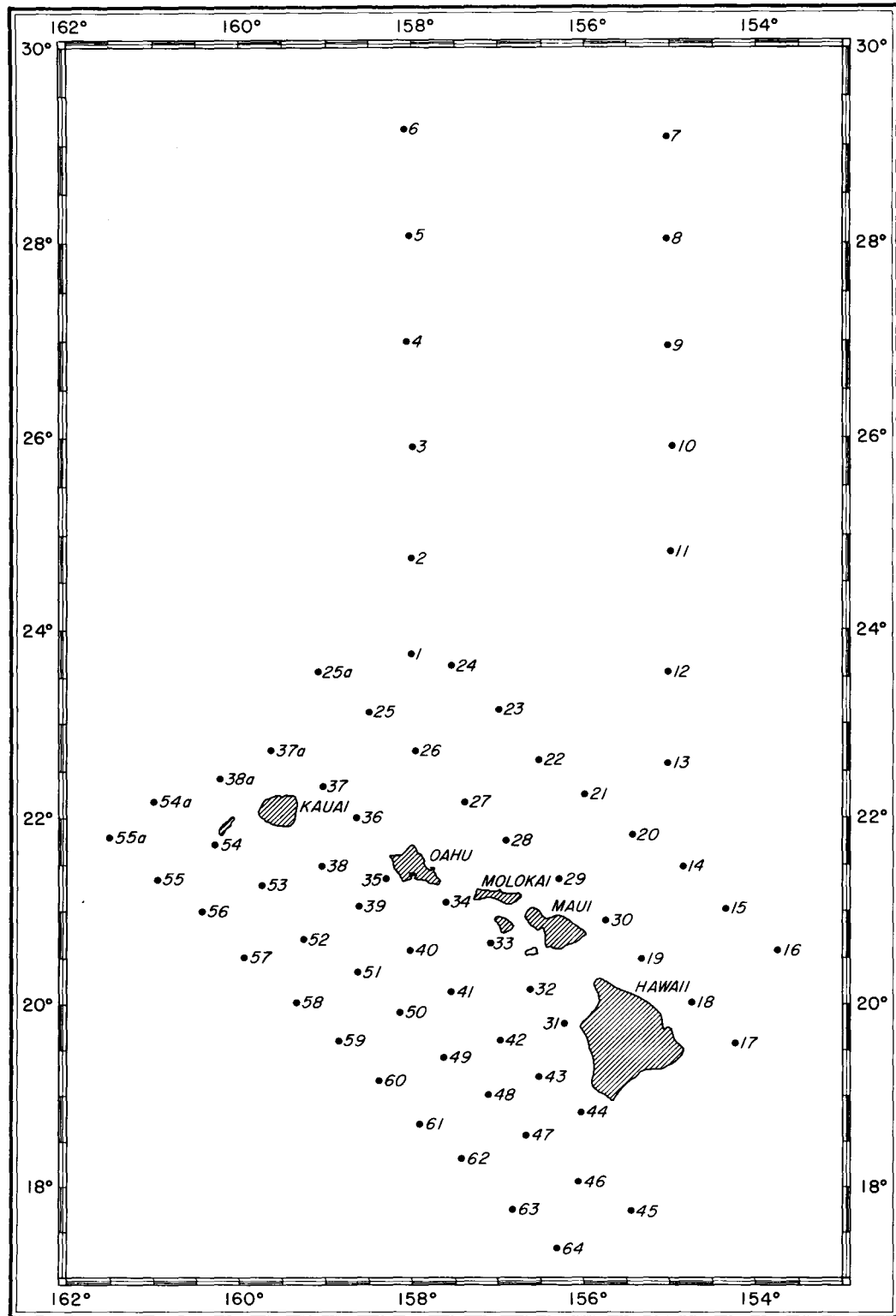
Figure 11. --Station positions, H. M. Smith cruise 20, March 1953.
