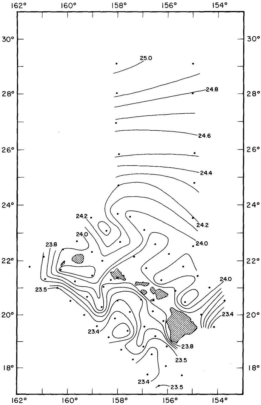
Figure 14.--Surface density ( \sigma_t ), H. M. Smith cruise 20, March 1953. Contour interval 0.1.
