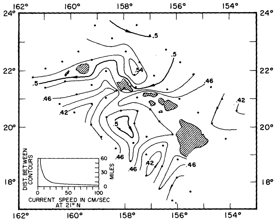
Figure 34.--Dynamic height anomalies (dynamic meters) at 250 m. relative to 500 m., H. M. Smith cruise 21, August 1953. Contour interval 0.02 dynamic meters.
