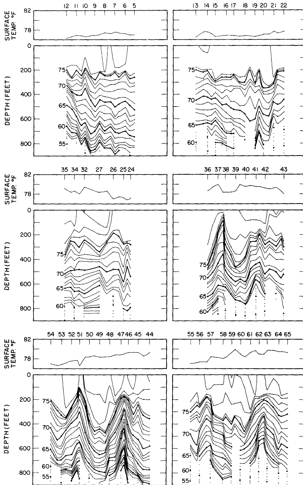
Figure 35.--Vertical bathythermograph temperature ( ^{\circ} F.) sections from stations 5 to 12, 22 to 13, 24 to 35, 43 to 36, 44 to 54, and 65 to 55, H. M. Smith cruise 21, August 1953. The upper panels show the surface bucket temperatures in ^{\circ} F.
