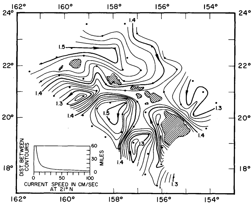
Figure 29.--Dynamic height anomalies (dynamic meters) at the surface relative to 500 m., H. M. Smith cruise 21, August 1953. Contour interval 0.02 dynamic meters.
