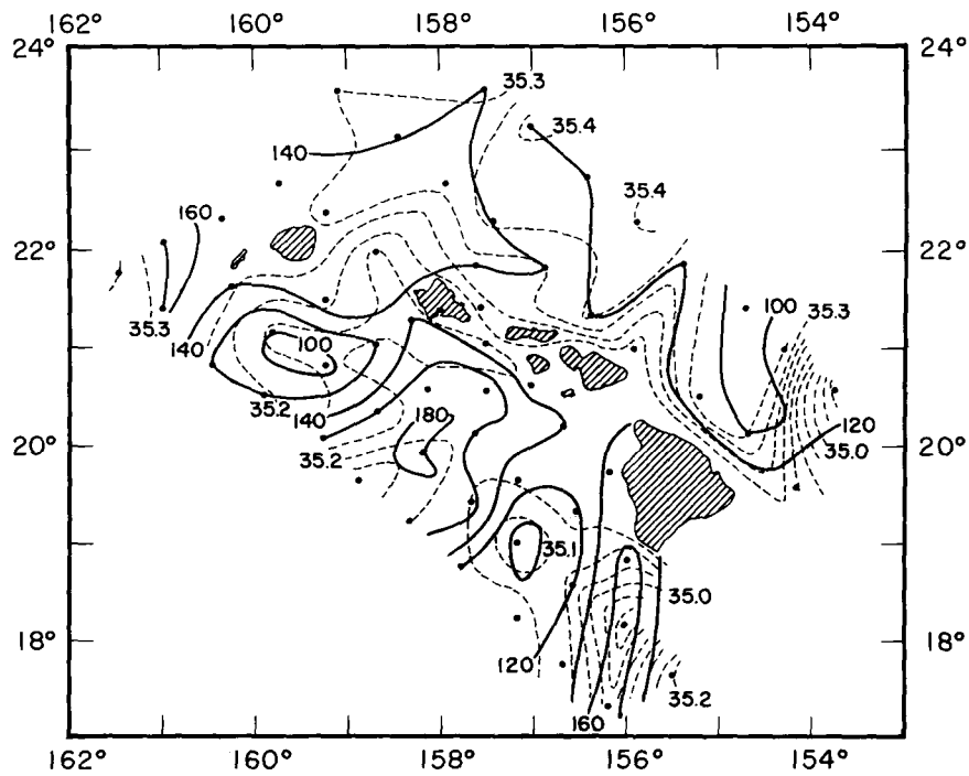
Figure 31.--Bathymetric chart (depth in meters) of the 24.5 sigma-t surface, H. M. Smith cruise 21, August 1953. Contour interval 20 m. Dashed lines indicate the salinity ( ^{\circ}/\infty ) distribution on the surface with contour intervals of 0.05^{\circ}/\infty .
