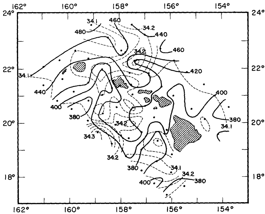
Figure 33.--Bathymetric chart (depth in meters) of the 26.5 sigma-t surface, H. M. Smith cruise 21, August 1953. Contour interval 20 m. Dashed lines indicate the salinity ( ^{\circ}/\text{oo} ) distribution on the surface with contour intervals of 0.05 ^{\circ}/\text{oo} .
