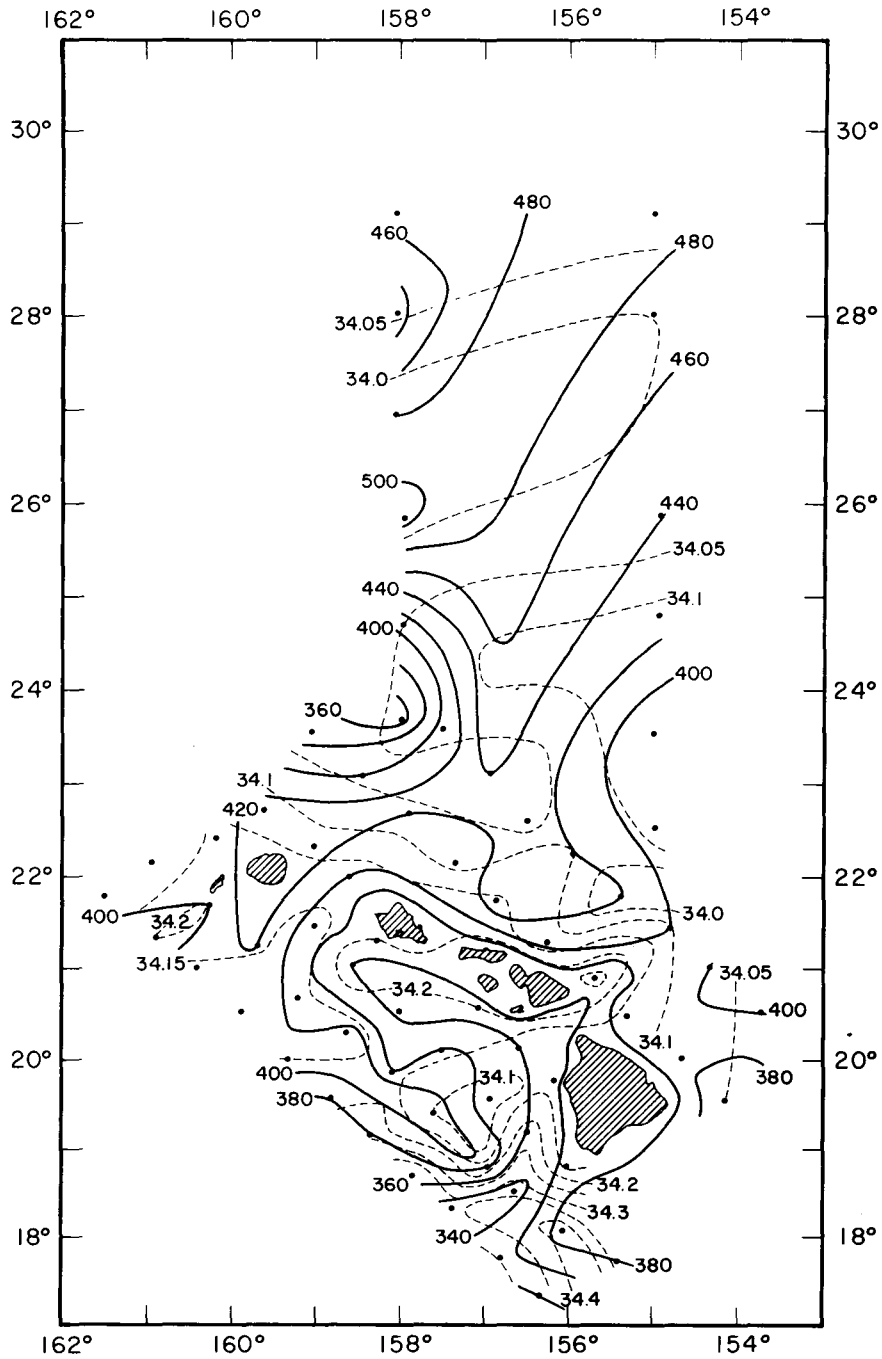
Figure 18. --Bathymetric chart (depth in meters) of the 26.5 sigma-t surface, H. M. Smith cruise 20, March 1953. Contour interval 20 m. Dashed lines indicate the salinity ( ^{\circ}/\infty ) distribution on the surface with contour intervals of 0.05^{\circ}/\infty .
