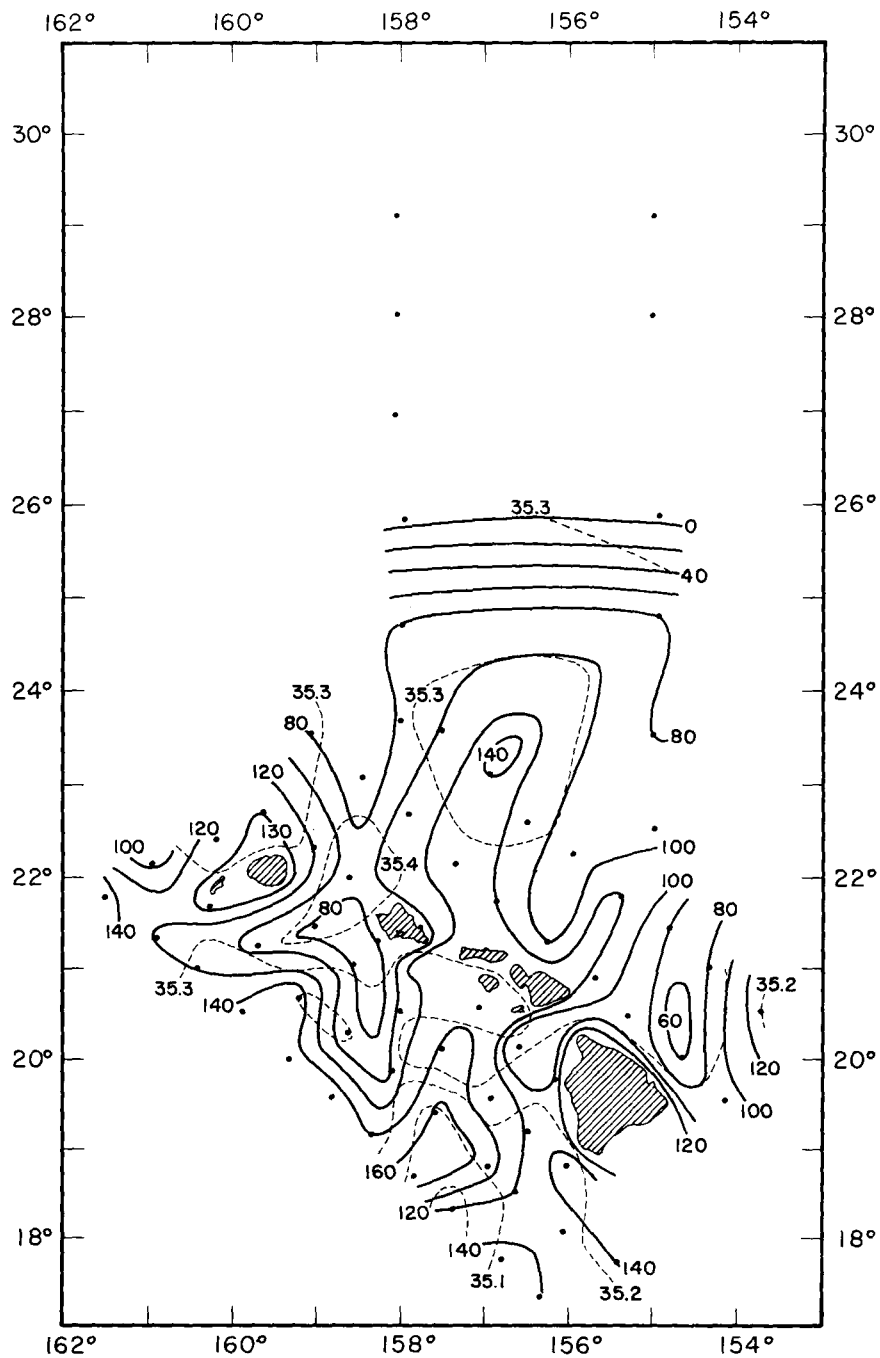
Figure 17. --Bathymetric chart (depth in meters) of the 24.5 sigma-t surface, H. M. Smith cruise 20, March 1953. Contour interval 20 m. Dashed lines indicate the salinity (‰) distribution on the surface with contour intervals of 0.1 ‰.
