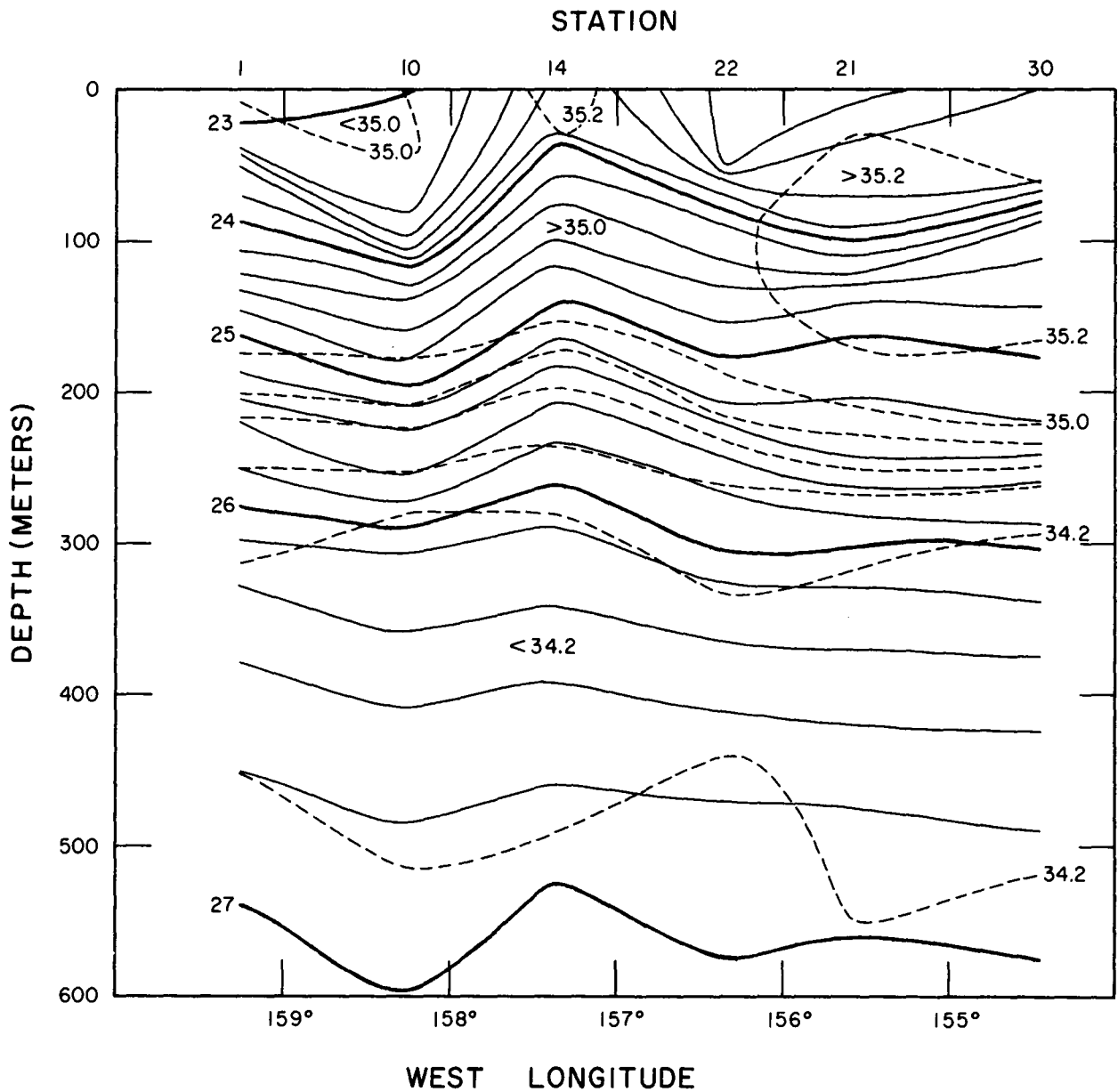
Figure 6. --Density ( \sigma_t ) section (solid lines) and salinity ( ^{\circ}/\text{oo} ) section (dashed lines) through stations 1, 10, 14, 22, 21, and 30, H. M. Smith cruise 17, September 1952. Sigma-t contour interval is 0.2, salinity contour interval 0.2 ^{\circ}/\text{oo} .
