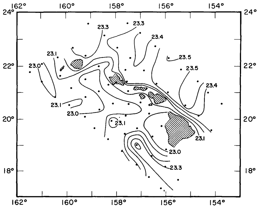
Figure 28.--Surface density ( \sigma_t ), H. M. Smith cruise 21, August 1953. Contour interval 0.1.
