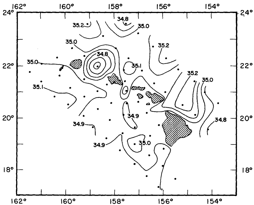
Figure 27.--Surface salinity in ^{\circ}/\text{oo} , H. M. Smith cruise 21, August 1953. Contour interval 0.1^{\circ}/\text{oo} .
