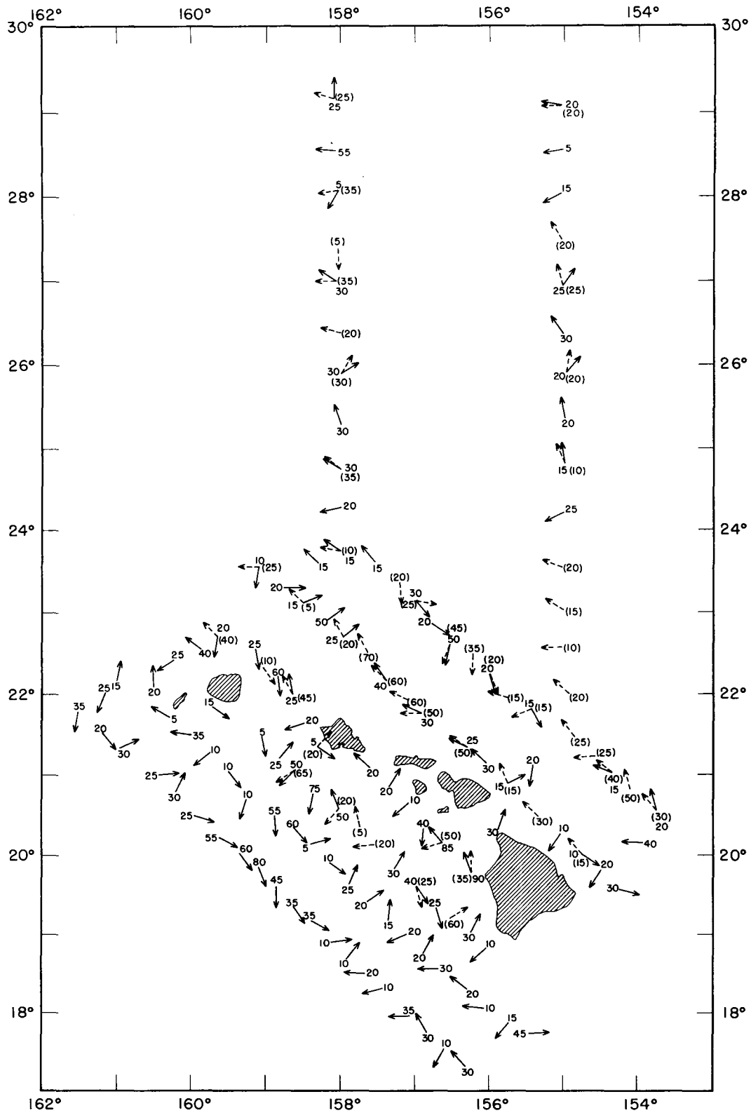
Figure 16. --Geomagnetic electrokinetograph (GEK) current speeds in cm./sec. and directions, H. M. Smith cruise 20, March 1953. Dashed arrows and numbers in parentheses indicate observations with floated electrodes.
