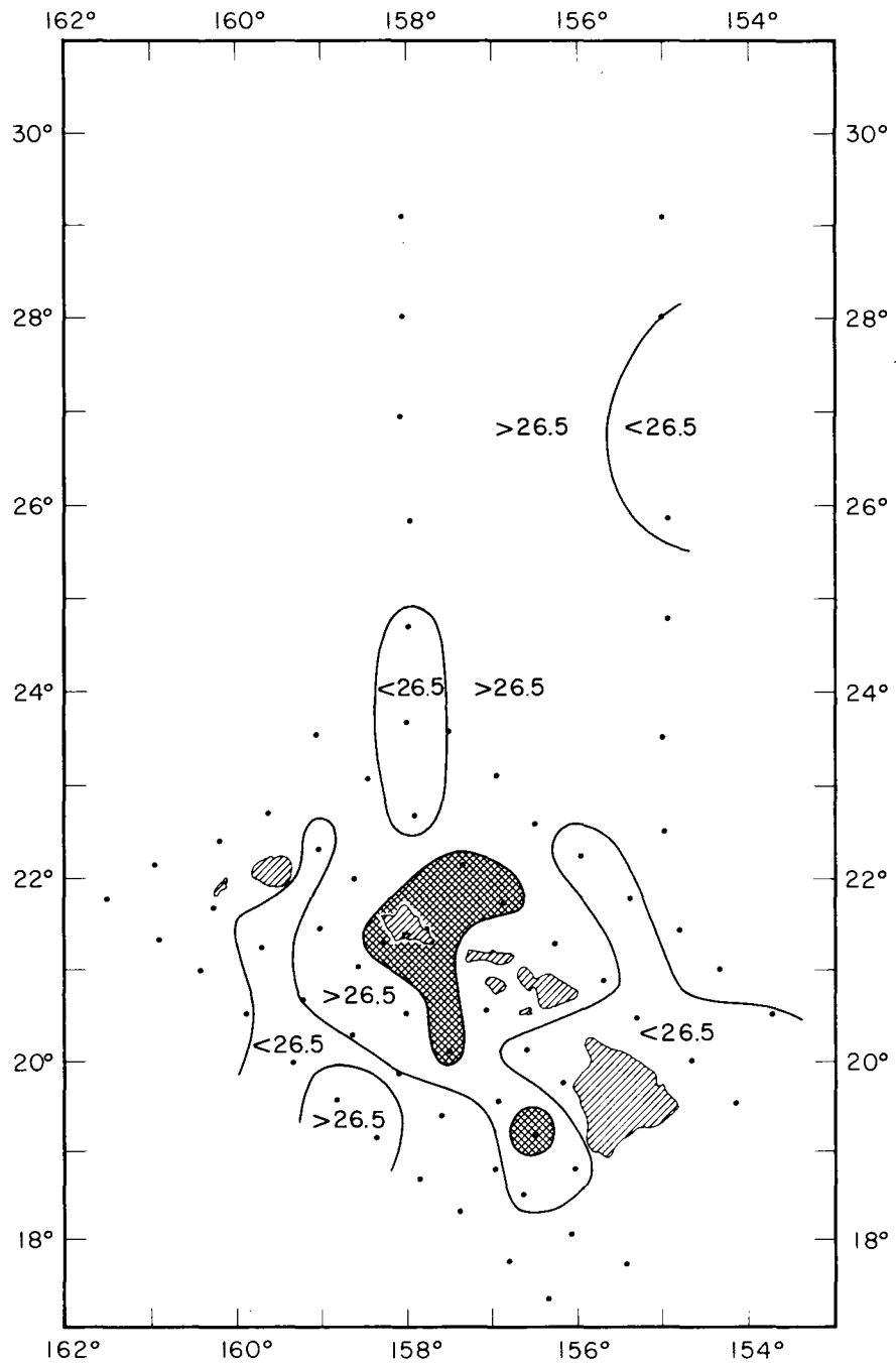
Figure 23.--Schematic diagram of the density ( \sigma_t ) distribution on the salinity minimum layer separated into regions where the \sigma_t is greater and less than 26.5. H. M. Smith cruise 20, March 1953. Cross-hatched zones include stations of constant salinity throughout a \sigma_t range of 26.1 to 26.8.
