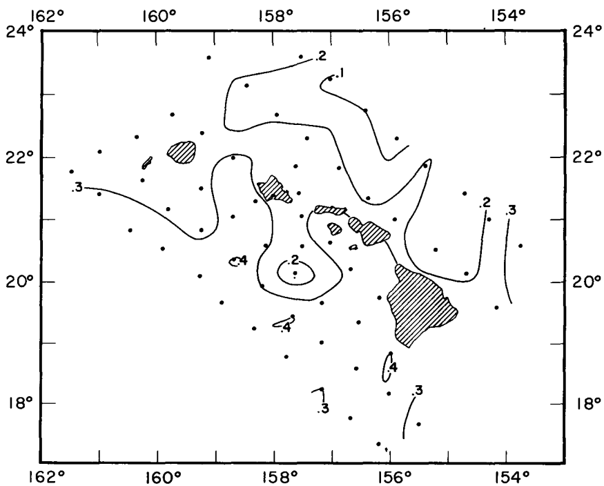
Figure 37. --Phosphate-phosphorus distribution ( \mu\text{g-at/l} ) on the 24.5 \sigma\text{-t} surface, H. M. Smith cruise 21, August 1953. Contour interval 0.1 \mu\text{g-at/l} .
