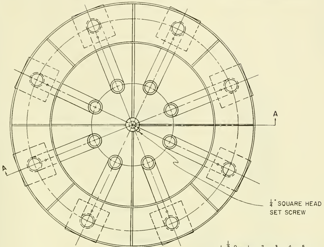
TOP SECTION FILTERING PAN
