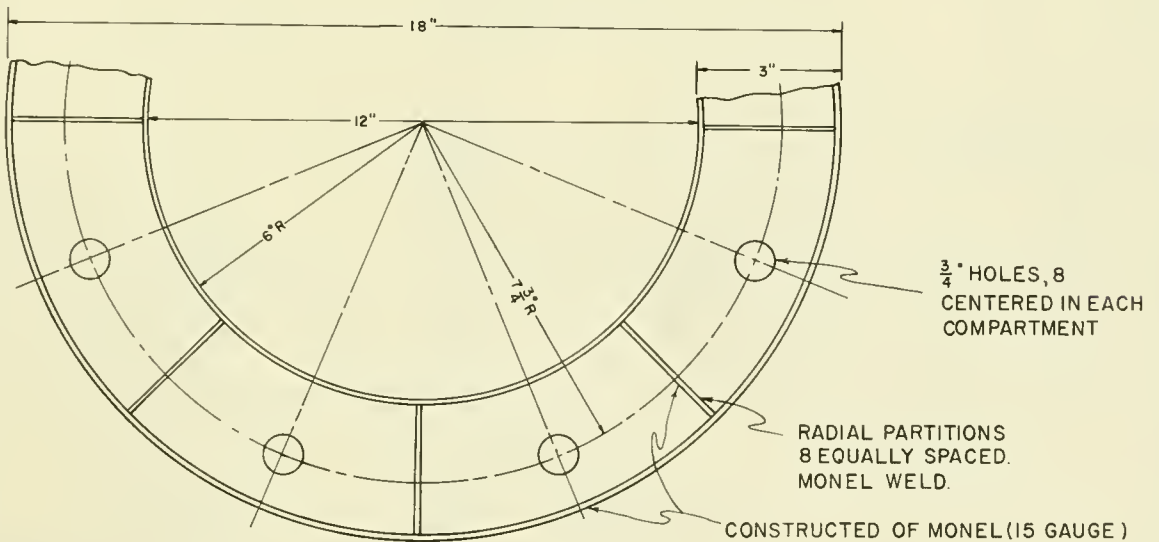
DETAIL FILTERING PAN
