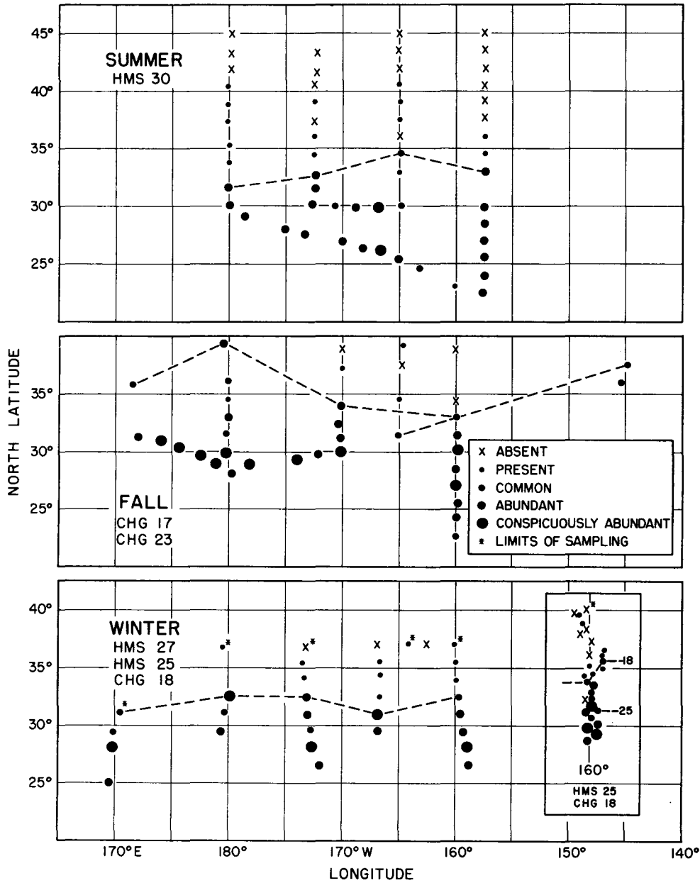
Figure 2. -- Seasonal variation in the northern limits of the Subtropic Zone (dashed line) as defined by the abundance of Pterosagitta draco . The symbols indicate the relative abundance of this species at each station where it occurred in the plankton collections.
