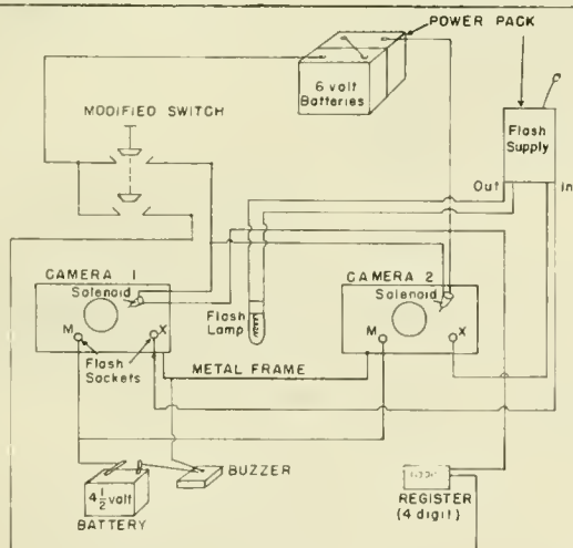
Figure 16 --Block diagram of wiring system.
