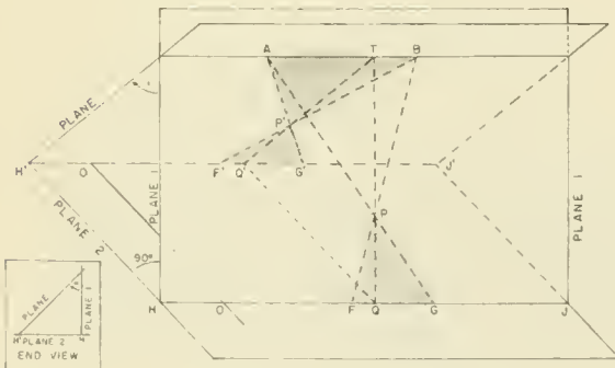
Figure 4. Locating point Q, the perpendicular projection of P', a point that is anywhere above plane 2 and that is in the field of view of the cameras at points A and B.
