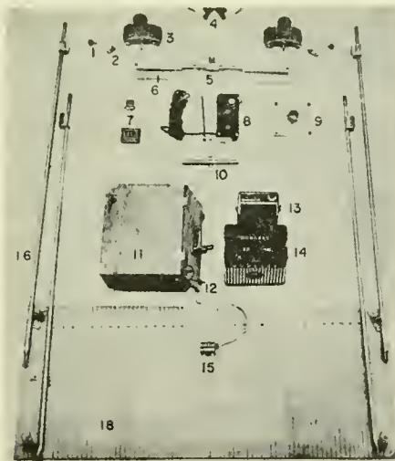
Figure 11.--Exploded view of photographic measuring device. (1) Rubber stops that keep cross member #1 firmly seated in the slots (as shown in Figures 12 and 13); (2) solenoids; (3) cameras; (4) cap and pins that hold legs firmly seated in the receptacles of the cap; (5) cross member #1; (6) adjustment washers that affords adjustment of the endwise rotation of the cameras; (7) bumper and bumper battery; (8) strobe light; (9) reflector; (10) cross member #2 with adjustment bolt that affords adjustment of the sideways rotation of the cameras; (11) battery box; (12) switch; (13) flash supply; (14) 6-volt batteries; (15) digital-register; (16) legs; (17) bolts used to attach legs to base; (18) base.
