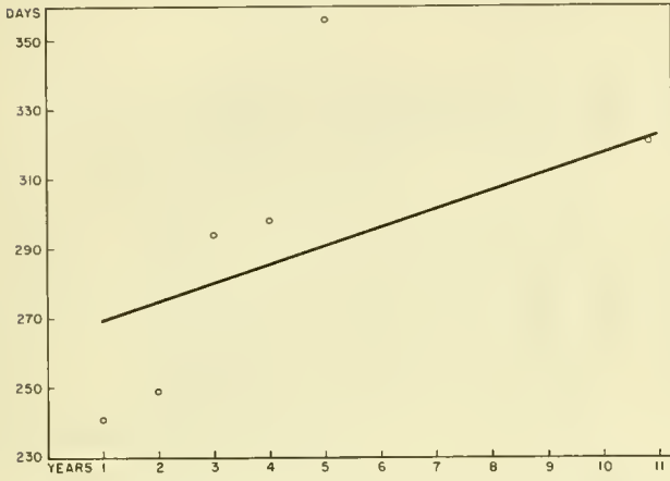
Figure 4.--Molt mid-dates; straight line fitted to data from table 6; female. ( Y = 264.05 + 5.46 X_1 )
