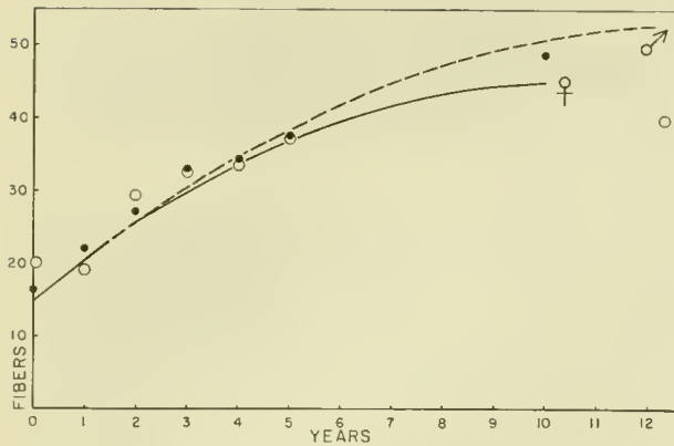
Figure 8.--Number of underfur fibers per bundle, by age and sex: quadratic curves fitted to the data of table 11. (Male, Y = 14.76 + 5.99 X - 0.236 X^2 ; female, Y = 14.89 + 5.90 X - 0.290 X^2 ).
