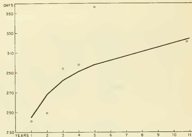
Figure 6.--Molt mid-dates; logarithmic curve fitted to data from table 6; female. ( Y = 245.40 + 75.65 \log X_1 )
