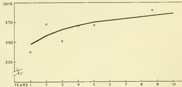
Figure 5.--Molt mid-dates; logarithmic curve fitted to data from table 6; male. ( Y = 248.41 + 30.27 \log X_1 )
