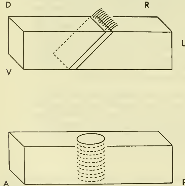
Figure 1.--Orientation of pelage samples, diagrammatic; body represented as lying on its belly with its head at viewer's left. D - V = dorsal to ventral axis; R - L = right to left axis; A - P = anterior to posterior axis. (Above) dry slice, transverse. (Below) ten paraffin mounts, horizontal.
