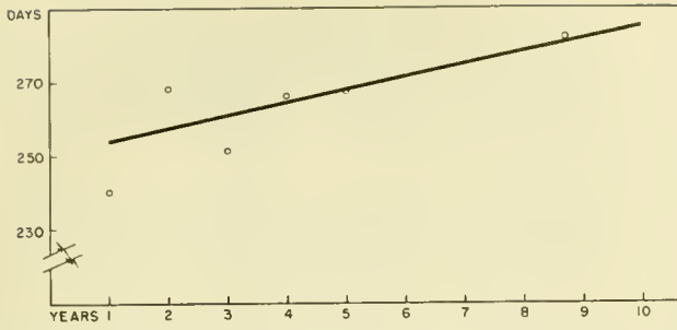
Figure 3.--Molt mid-dates; straight line fitted to data from table 6; male. ( Y = 250.55 + 3.43 X_1 )
