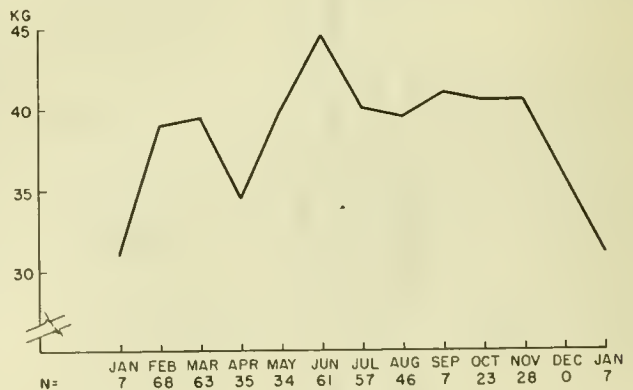
Figure 9.--Change in body weight of the female by month, based on 429 mature animals, age 11 years or older, not pregnant.
