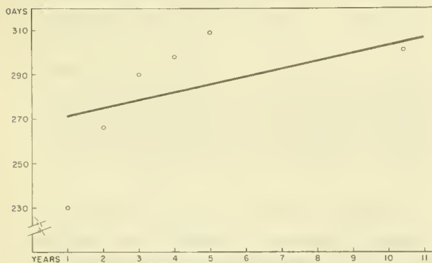
Figure 7.--Molt mid dates; straight line fitted to data from table 6; sexes combined. ( Y = 267.53 + 3.59X .)
