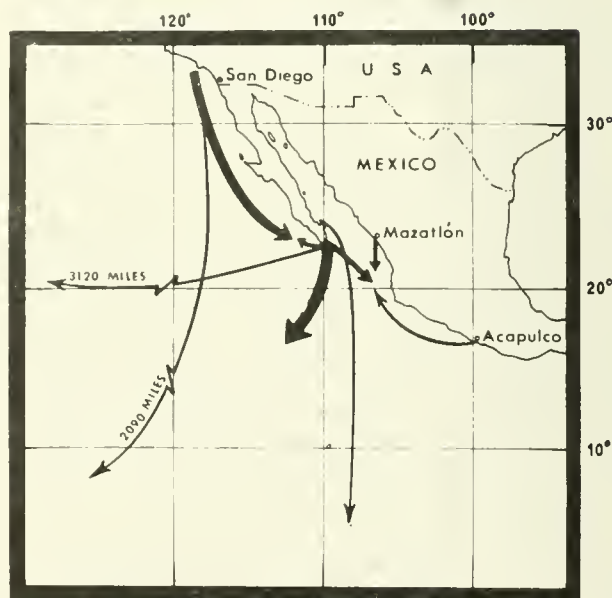
Figure 7.—General migration patterns of striped marlin tagged off southern California and Mexico.
