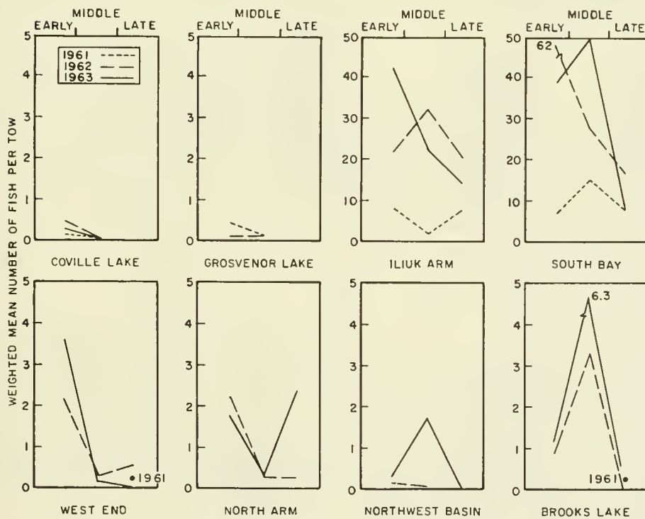
Figure 6.—Weighted mean number of age 1 sockeye salmon per standard tow by early, middle, and late time periods in each lake of the Naknek River system 1961-63.
