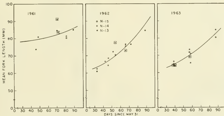
Figure 17.—Curves of apparent growth of age 1 sockeye salmon captured in tow nets in sampling units of Iliuk Arm, 1961-63.
