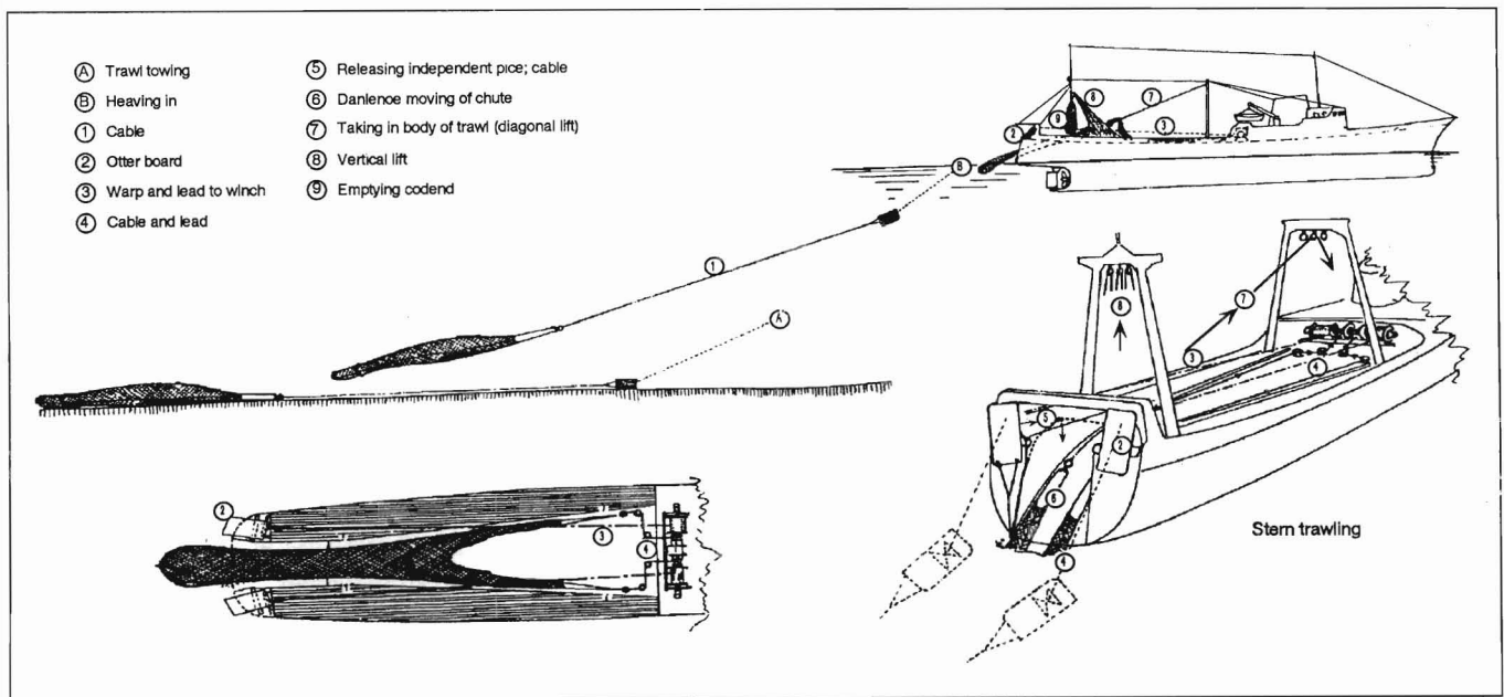
Figure 8 Method of heaving gear aboard a stern trawler (adapted from Garner 1967).
