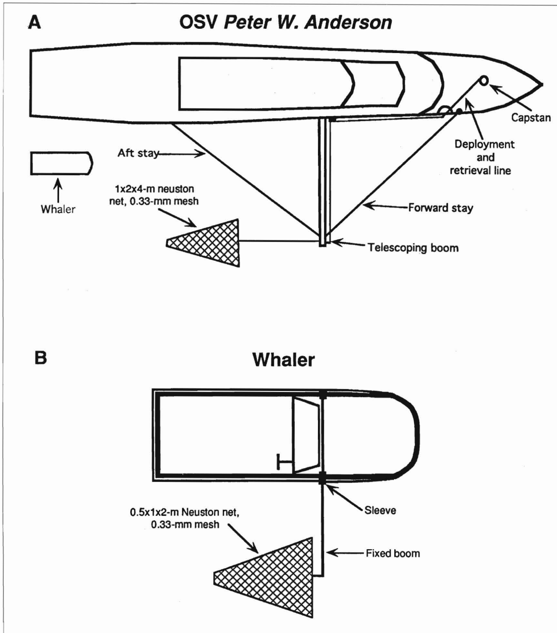
Figure 4 Example of sampling vessel equipped with telescoping boom (from the U.S. Environmental Protection Agency [1990b]).
