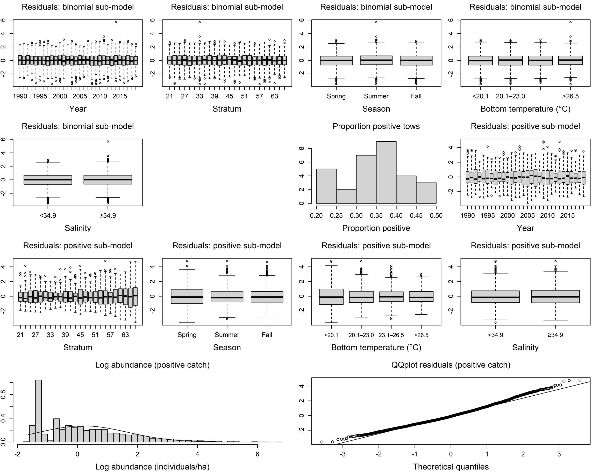
Supplementary Figure 2. Residuals and quantile plots based on the delta-GLM standardization of bluefish ( Pomatomus saltatrix ) abundance.
