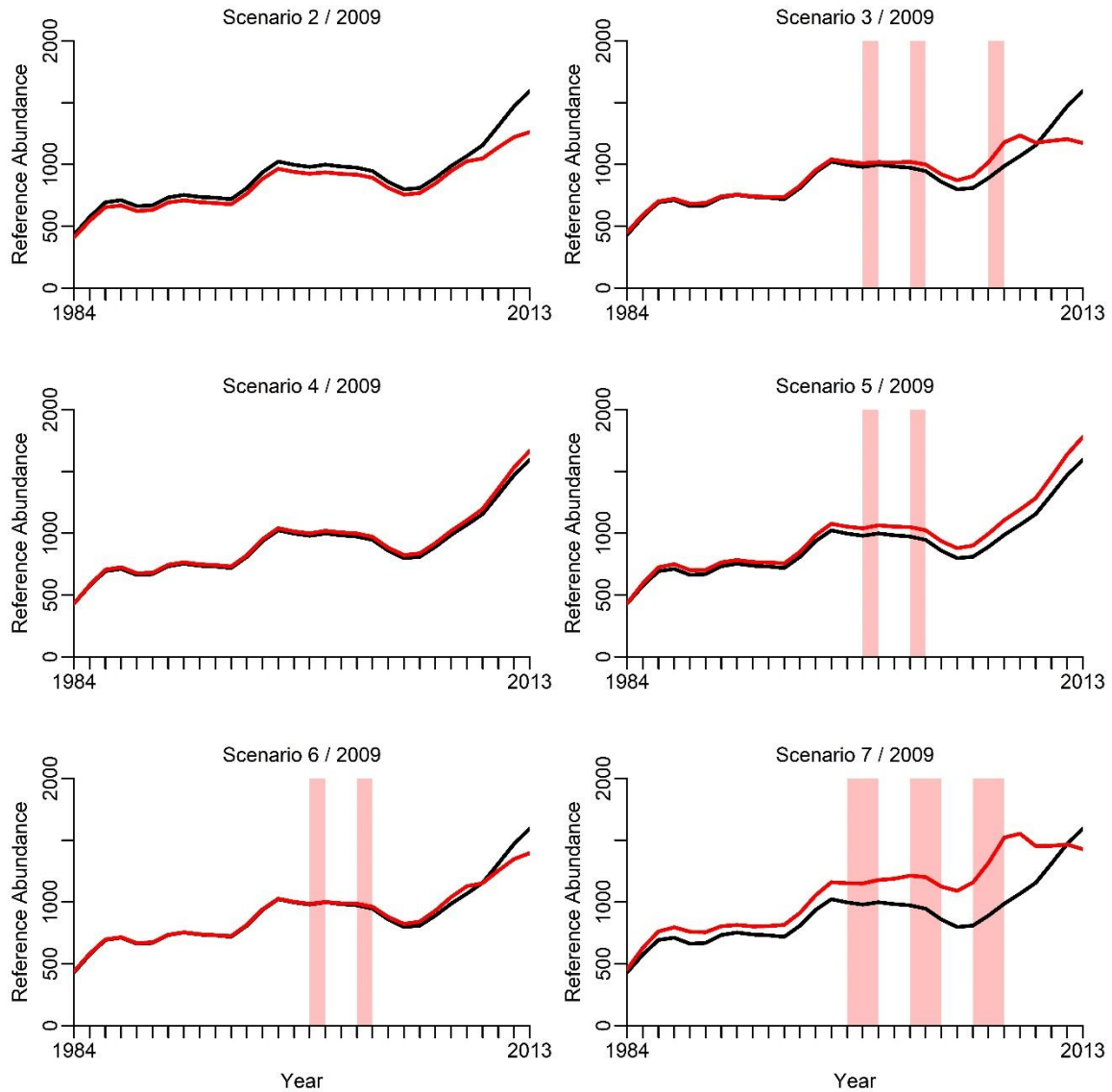
Supplementary Figure 1. Estimated reference abundance (in millions of individuals) 1984–2013 for University of Maine Model scenarios corresponding to those in Table 1 (red trend lines) compared to the base case (black trend lines). Note that the scenarios in Table 1 are only applied after a regime shift at 2009. Pre-2009 for all Runs 2–7 are with base case data, whereas post-2009 for all Runs 2–7 are using the growth matrices and size-at-maturity values that correspond with scenarios 2–7 in Table 1. Shaded regions indicate years where the historical fishery status is different from that of the base case for the same year. Note the differences in vertical axes ranges between plots. The results from this analysis agreed with the results of non-time varying growth and size-at-maturity data (Figure 2).
