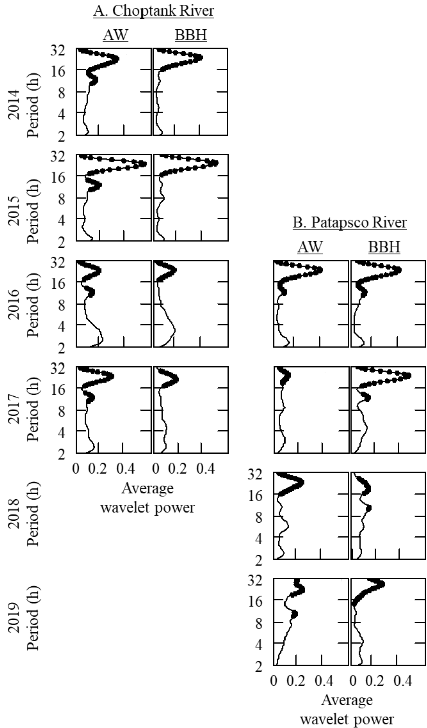
Supplementary Figure 7. Global spectra from wavelet analyses of hourly upstream estimates of alewife (AW) and blueback herring (BBH) each year in the Choptank River (2014-2017, A) and Patapsco River (2016-2019, B).
