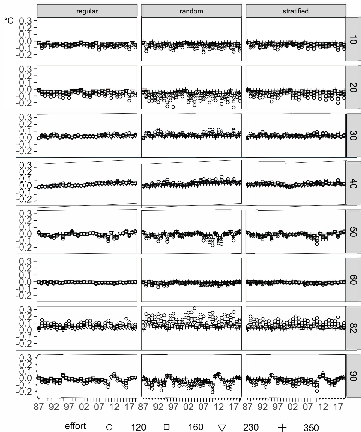
Supplementary Figure 1. Mean bias of eastern Bering Sea shelf bottom temperature ( ^{\circ}\text{C} ) prediction by sampling method and effort (number of stations) for each stratum and survey year (1987–2019).
