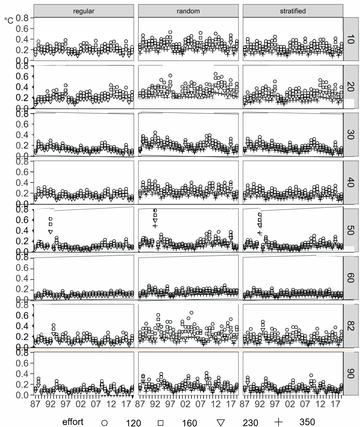
Supplementary Figure 2. Root mean squared error (RMSE) of eastern Bering Sea shelf bottom temperature ( ^{\circ}\text{C} ) prediction by sampling method and effort (number of stations) for each stratum and survey year (1987–2019).
