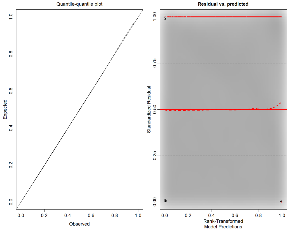
Supplementary Figure 2. Quantile-quantile plot (left) and residual plot (right) generated by the “DHARMa” package in R Statistical Software.
