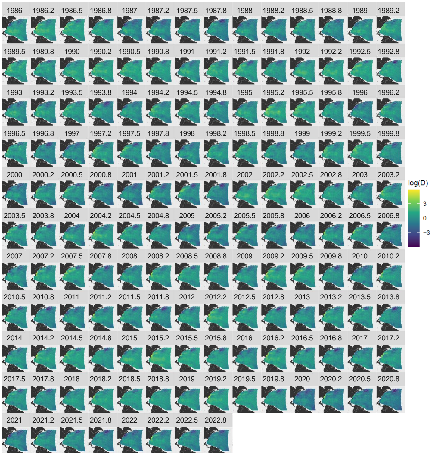
Supplementary Figure 3. Estimated log-scale dolphinfish ( Coryphaena hippurus ) density (D) plots over space and time. The space over which log-scale densities were estimated represents the custom extrapolation grid described in the Methods. Log-scale density estimates are provided by both year and season, which is denoted with a decimal number after the year, e.g., “2012.2”; no decimal after the year indicates the winter season, “.2” indicates the spring season, “.5” indicates the summer season, and “.8” indicates the fall season.
