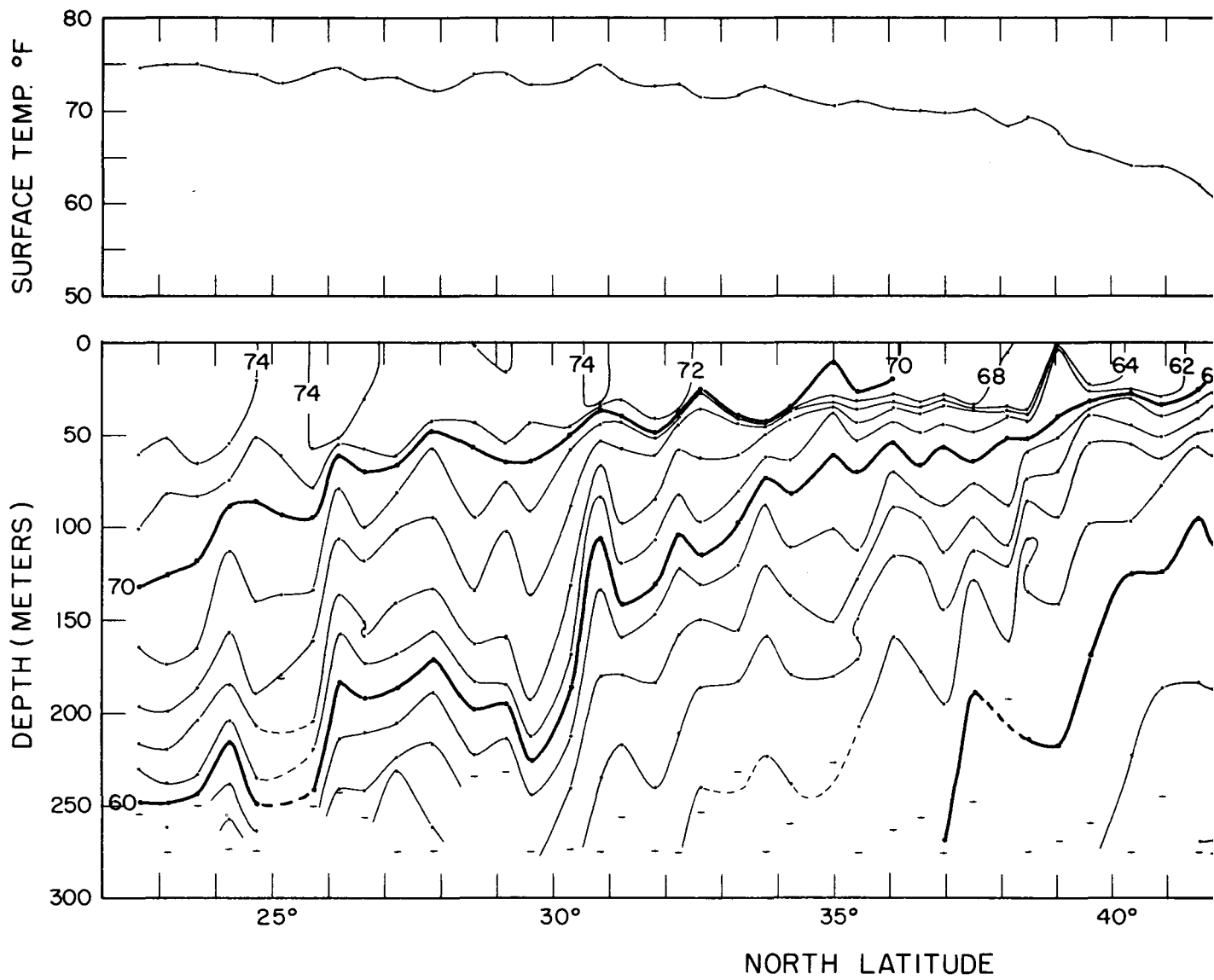
Fig. 8.--Surface bucket temperatures (upper panel) and temperature-depth section from BT observations (lower panel). Section A (see figure 7), JRM Cruise 26, July-September 1955.
