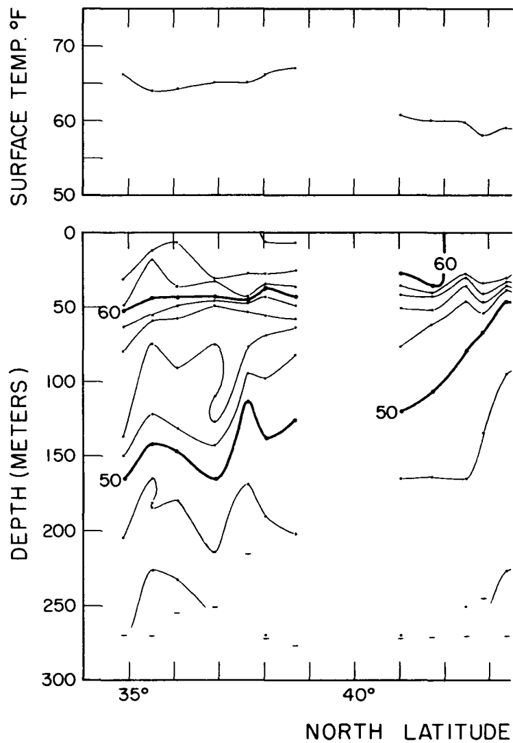
Figs. 9 (left) and 10(right). --: observations (lower panels)
