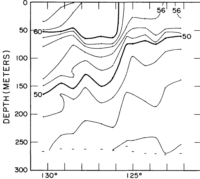
Surface bucket temperatures (upper panels) and temperature-depth sections from BT . Sections B and C (see figure 7), JRM Cruise 26, July-September 1955.
