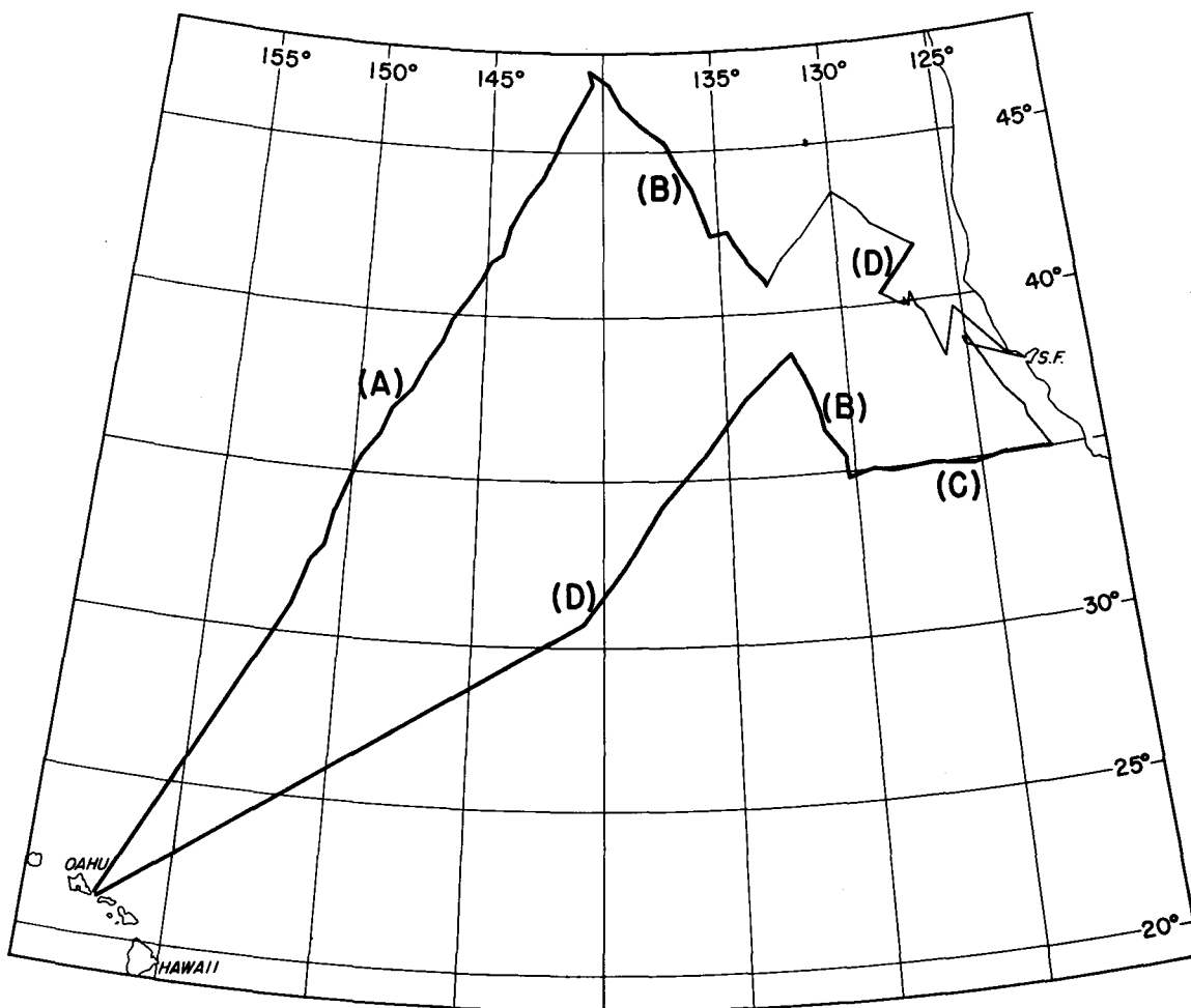
Fig. 7.--Track chart, JRM Cruise 26, July-September 1955. Heavy lines and letters designate location of temperature sections shown in figures 8 to 11.
