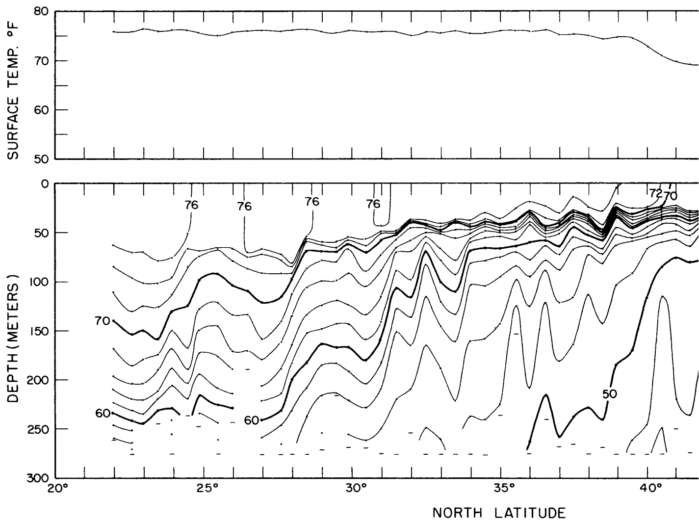
Fig. 6.--Surface bucket temperatures (upper panel) and temperature-depth section from BT observations (lower panel). 157°W. longitude; HMS Cruise 30 (NORPAC), July-August 1955.
