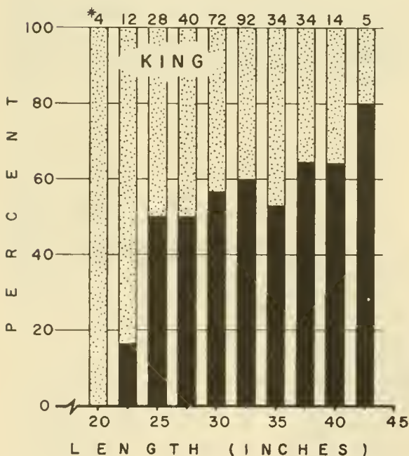
Figure 5.--Percentage frequency of occurrence in relation to length of salmon (by 2.5-inch intervals) of food items taken from stomachs of troll-caught salmon, South-eastern Alaska, 1957-58.
