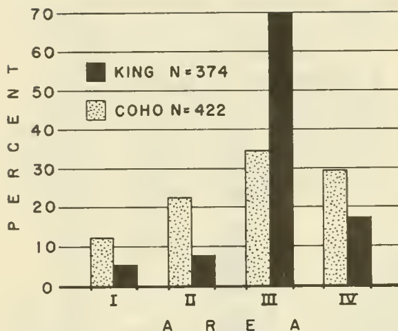
Figure 2.--Percentages of stomach samples from troll-caught salmon by area, Southeastern Alaska, 1957-58. [Areas shown in figure 1.]
