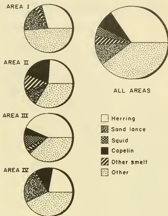
Figure 3.--Frequency of occurrence of major items found in salmon stomachs, Southeastern Alaska, 1957-58. [Based on total occurrence of food items.]
