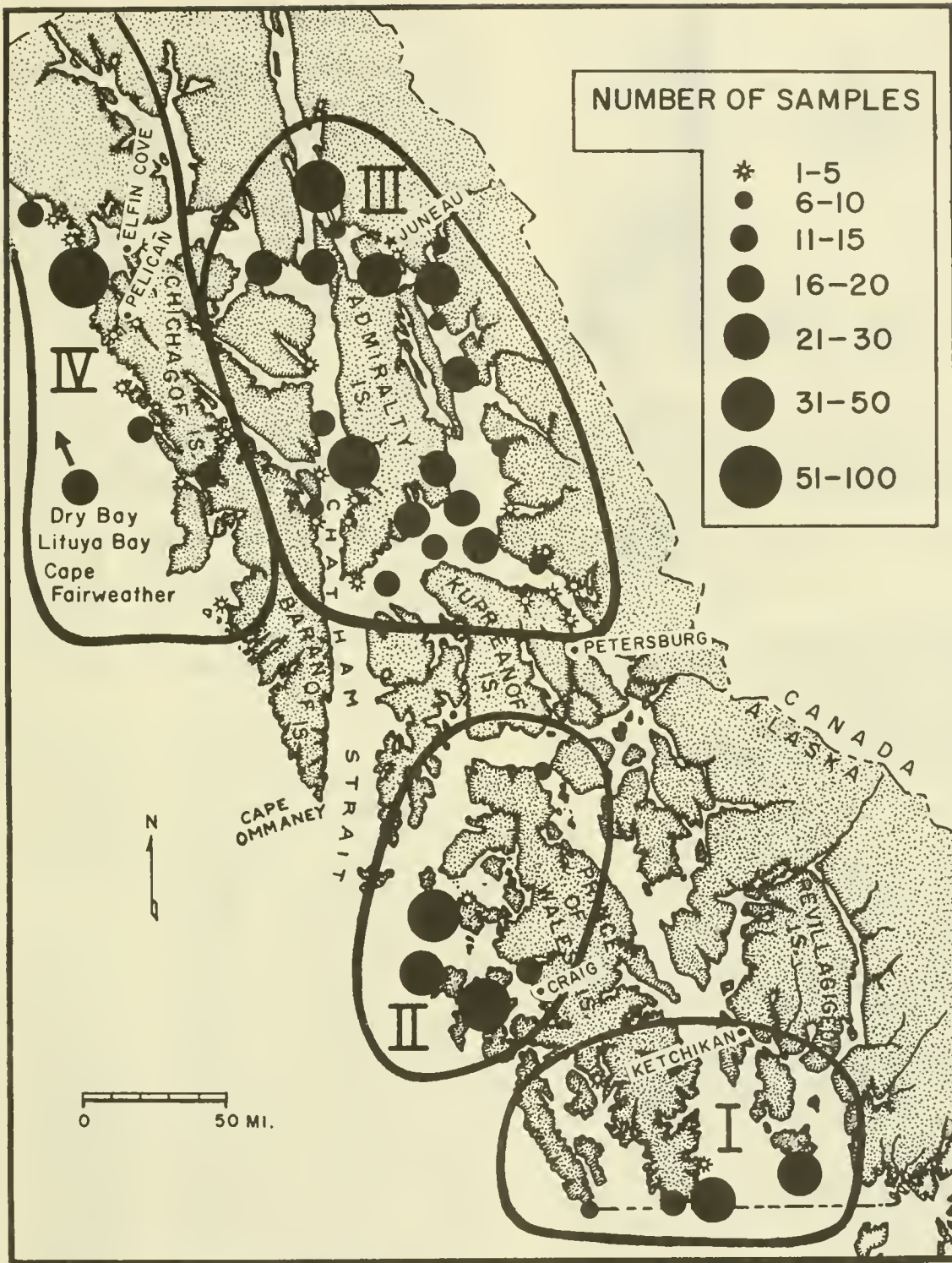
Figure 1.--Locations of capture of king and coho salmon from which stomach samples were taken in Southeastern Alaska, 1957-58.
