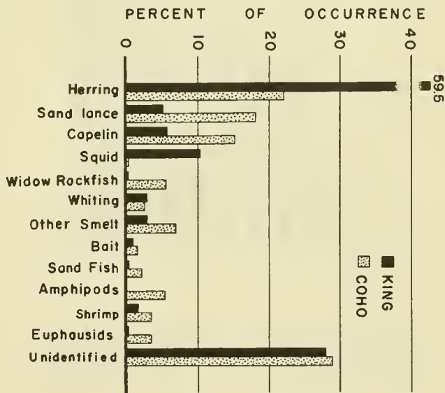
Figure 4.--Percentage frequency of occurrence of food items found in stomach samples from king and coho salmon in Southeastern Alaska, 1957-58. [Percentages based on stomachs containing food.]
