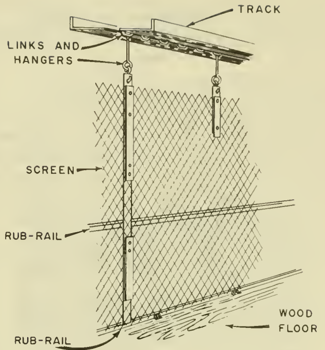
Figure 4.--Screen and 25-mm. flat bracket attachments.
