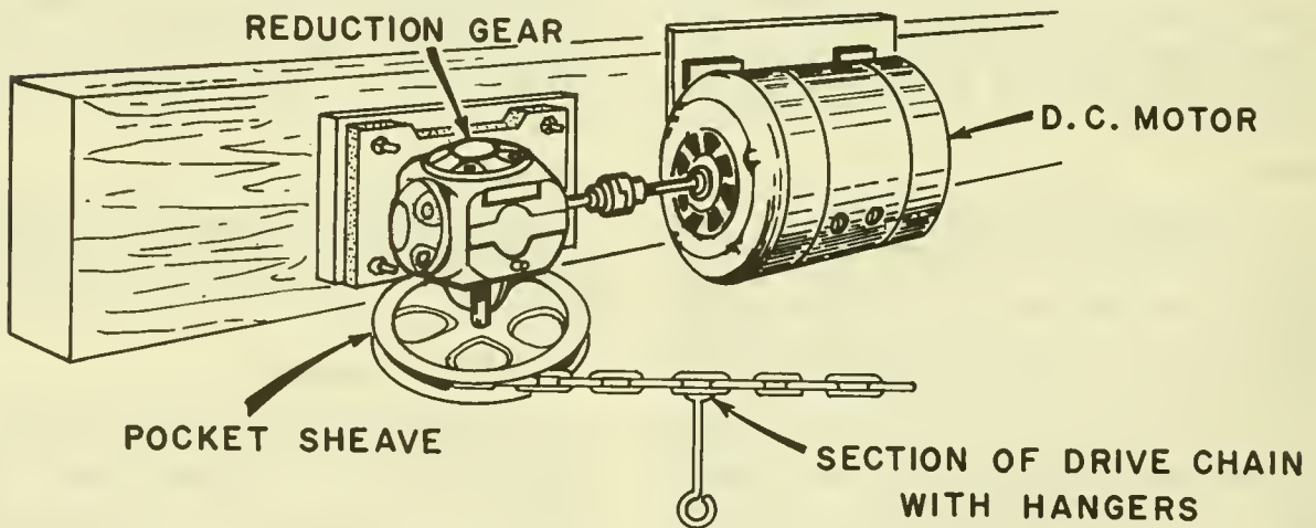
Figure 2.--Variable-speed d.c. motor and reduction gear drive assembly on travelling screen.
