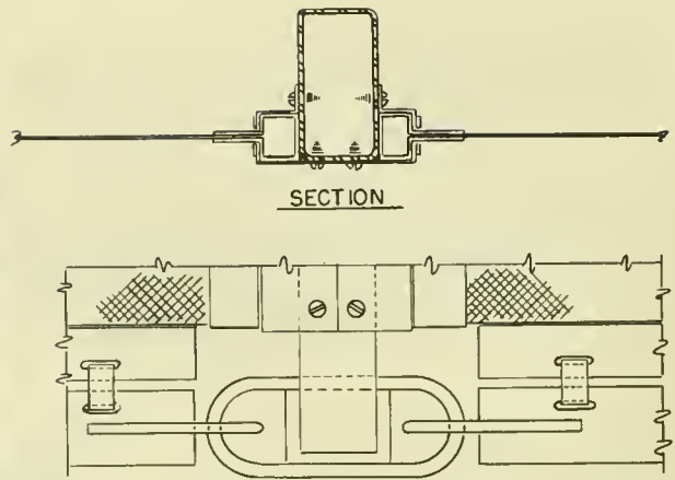
Figure 10.--Corner joint of screen panel.
