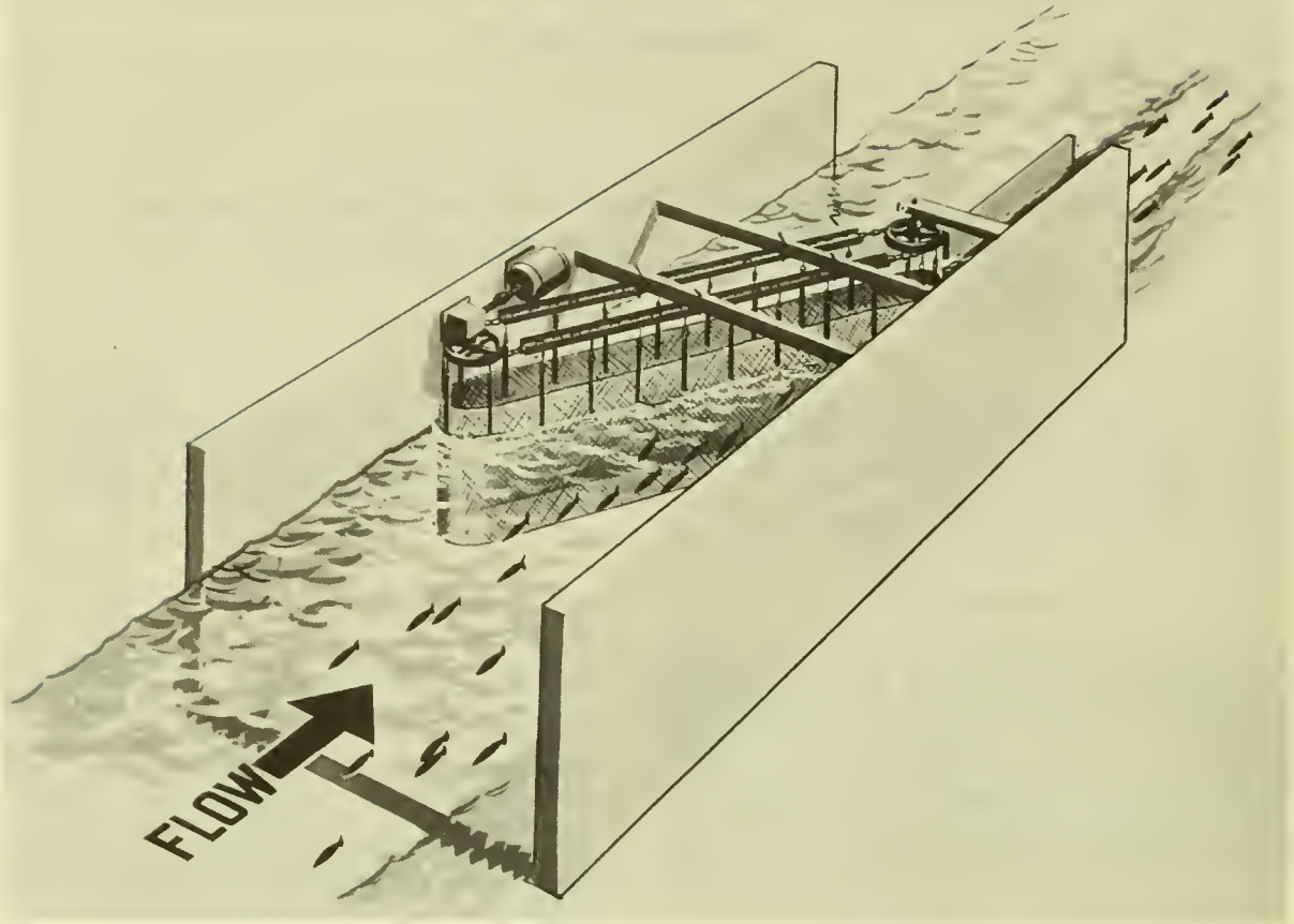
Figure 1.--Horizontal travelling screen, model I.
