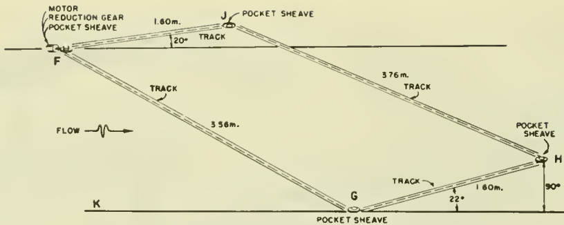
Figure 6.--Horizontal travelling screen, model II.
