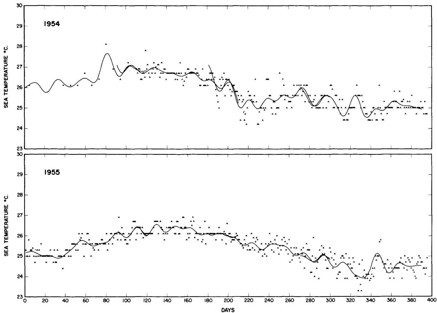
APPENDIX D FIGURE 1.—Sea-surface temperatures, Christmas Island, 1954-69.
