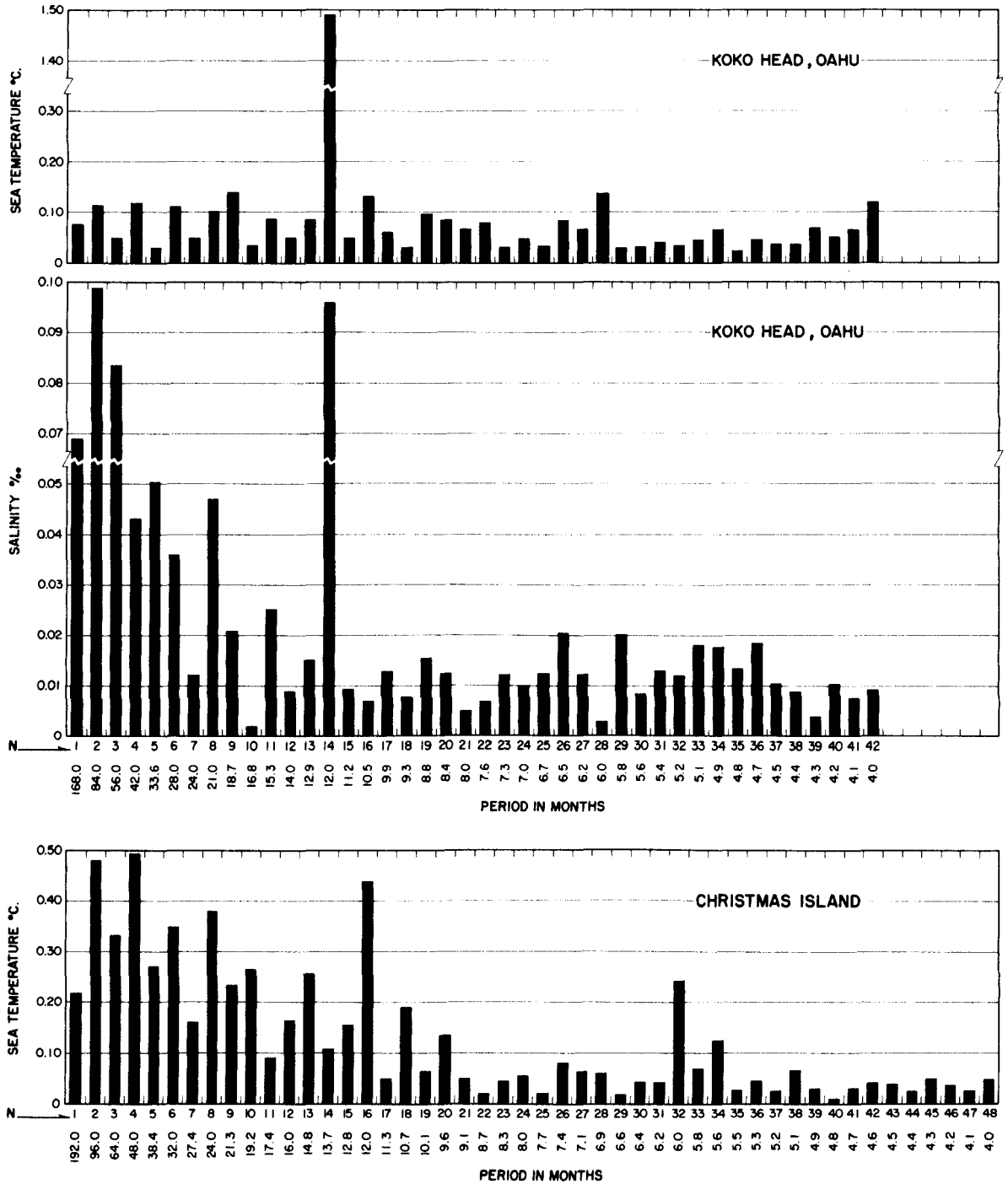
FIGURE 4.—Spectra of the long-term harmonic functions for Koko Head temperatures, 1956-69, Koko Head salinities, 1956-69, and Christmas Island temperatures, 1954-69.
