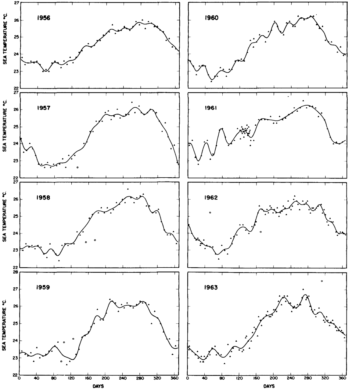
APPENDIX B FIGURE 1.—Sea-surface temperatures, Koko Head, 1956-69.
