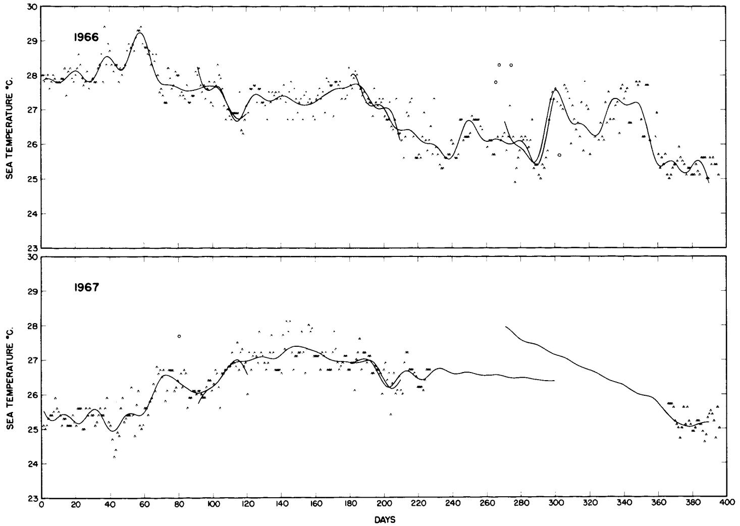
APPENDIX D FIGURE 1.—Sea-surface temperatures, Christmas Island, 1954-69.—Continued.
