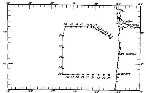
FIGURE 4.—Location of STD (Salinity-Temperature-Depth probe) stations during the pre-season albacore cruise, 7-10 July 1970. (Cayuse 7007A).
