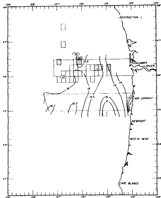
FIGURE 9.—Sea-surface temperatures and albacore catch rates, 30 July 1970. See Figure 6 for explanation of catch notation.
