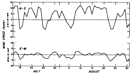
FIGURE 3.—Components of average daily wind velocities recorded at Newport, Oreg.
