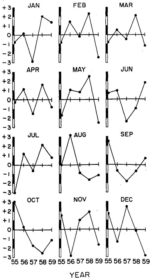
FIGURE 10.—Graphs of principal components of upwelling index for the CalCOFI survey area for each month for the years 1955-59. See text and Bakun (1973).
