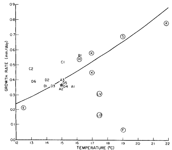
FIGURE 3.—Relationship between growth rate (millimeters/day at 8 mm) and temperature for northern anchovy larvae from the field (bare symbols) and in the laboratory (circled symbols). Field samples, this study, A1-D6; composite of nine field samples, B1, C1, and C2 not included, ☆; Hunter 1976, laboratory-reared prey, H; Kramer and Zweifel 1970, wild plankton for food, K; Lasker et al. 1970, dinoflagellates only, LD, dinoflagellates plus veliger, LV; Sakagawa and Kimura 1976, S; unpubl. data available at Southwest Fisheries Center, low temperature experiment, E, periodic starvation experiment, F. Curve was derived from the model of Zweifel and Hunter (see text footnote 2); it was not fit to the growth rate data presented here.
