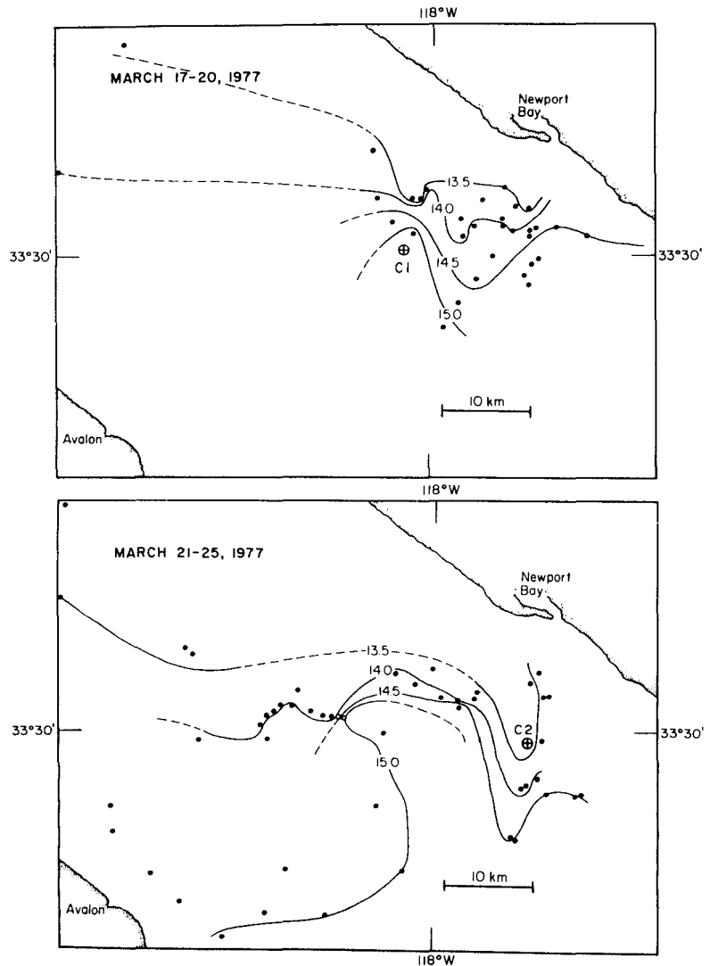
FIGURE 4.—Surface isotherms in degrees Celsius between Los Angeles and Santa Catalina Island, Calif., in March 1977.
