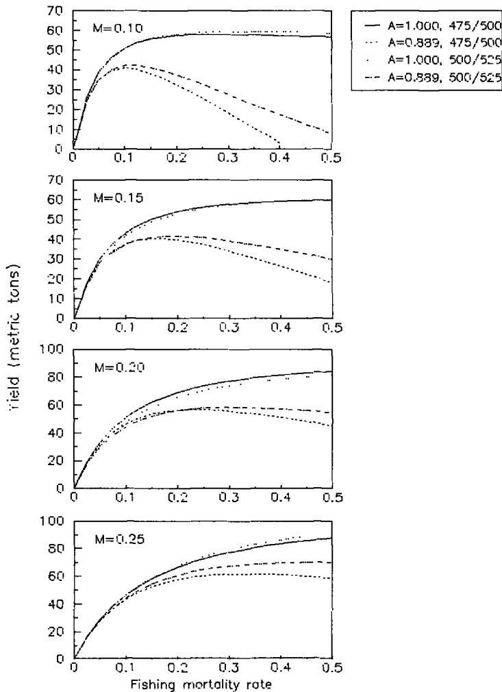
FIGURE 4.—Estimated equilibrium yield at four rates of natural mortality ( M ), two assumptions regarding the stock-recruitment relationship ( A = 0.889 - recruitment dependent on spawning stock, A = 1.000 - recruitment constant), and two values for the female and male ( F/M ) selectivity parameter L50_{sel} .
