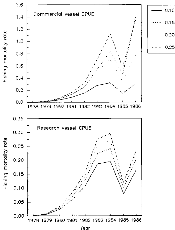
FIGURE 3.—Estimated fishing mortality rates ( F ) from 1978 to 1986 at natural mortality rates of 0.10–0.25. At each level of natural mortality, the virgin recruitment level was determined based on the correlation between F and estimated fishing effort, where estimates of effort were based on commercial vessel or research vessel CPUE. Results for the alternative set of selectivity parameters ( L_{50_{S_d}} ) were similar and are not shown here.
