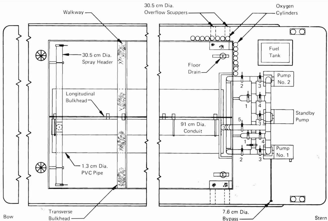
Figure 3.—Overhead view of a fish barge (modified from U.S. Army Corps of Engineers' blueprint). Key to valves: 1) Sea chest, 2) Recirculation, 3) Pump intake, 4) Back flush, and 5) Main discharge.
