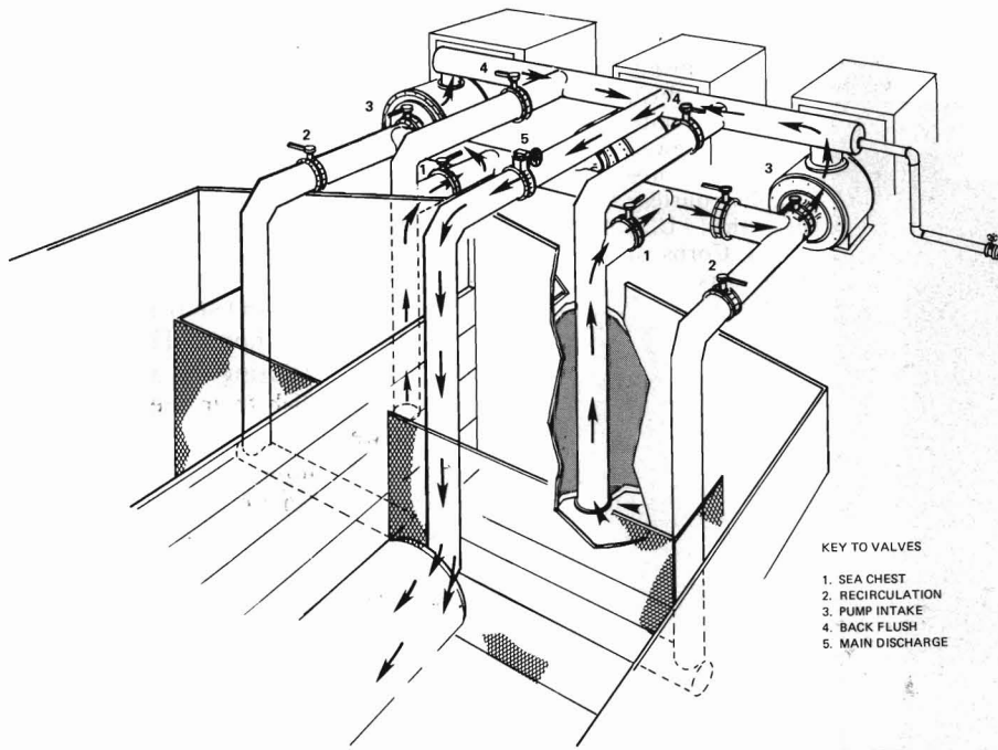
Figure 4.—Diagram of the stern plumbing on the fish barge: Arrows indicate water flow during normal circulation. Valve handles parallel to the flow indicate open valves.
