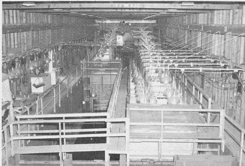
FIGURE 4.—View from the upper turn pool showing respective lengths of the 1-on-16 (right) and 1-on-8-slope (left) fishways. Each fishway rises 16 feet.
