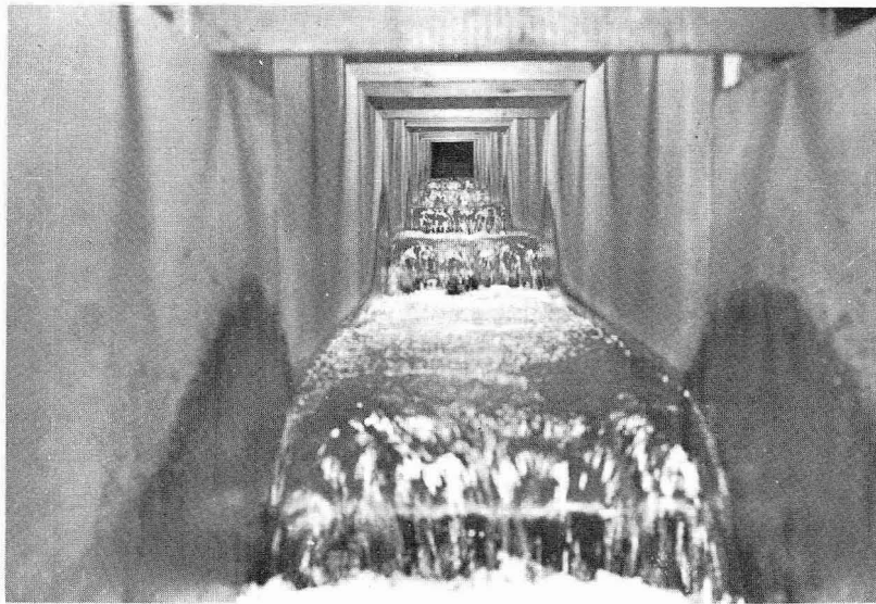
FIGURE 6.—The 1-on-16-slope endless fishway viewed from pool 53.
