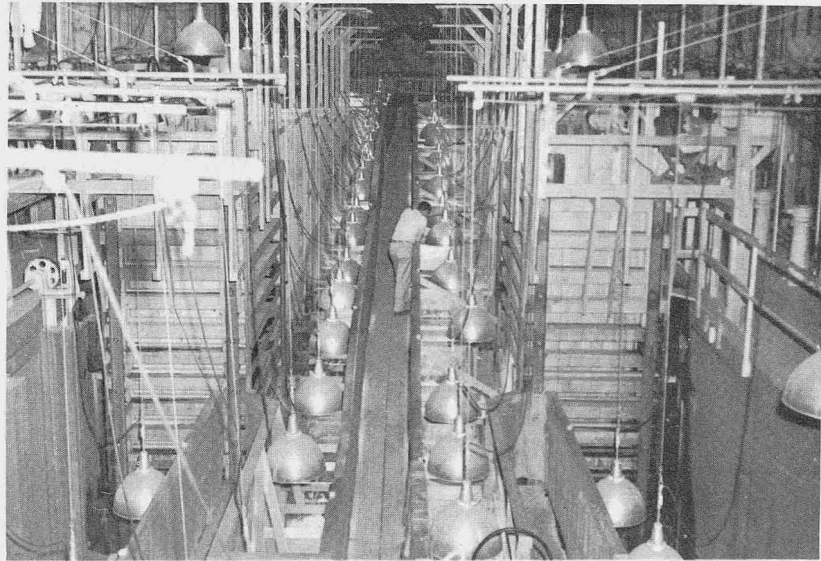
FIGURE 3.—Looking upstream at the 1-on-16 (left) and 1-on-8-slope (right) endless fishways. The locking units in each fishway appear in the left and right foreground.
