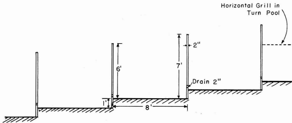
FIGURE 7.—Sectional view of 1-on-8-slope fishway. Note level floors.
