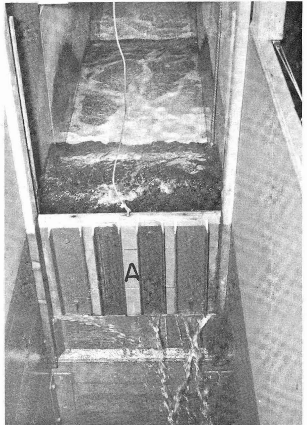
FIGURE 11.—Drop gate (A) in down position separating diffusion chamber from lock (foreground). Water in lock (foreground) has been discharged to elevation 51'.
