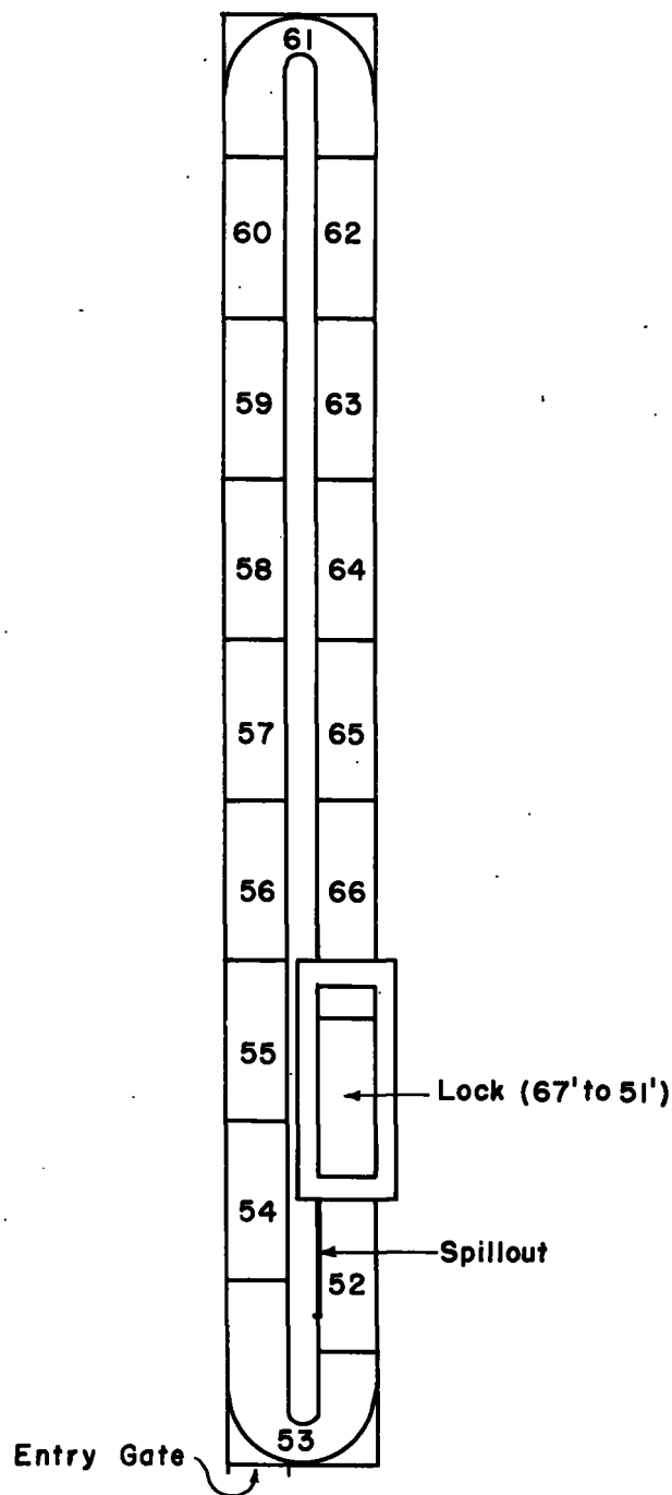
FIGURE 2.—Plan view of 1-on-8-slope fishway showing pool elevations in height above mean sea level.
