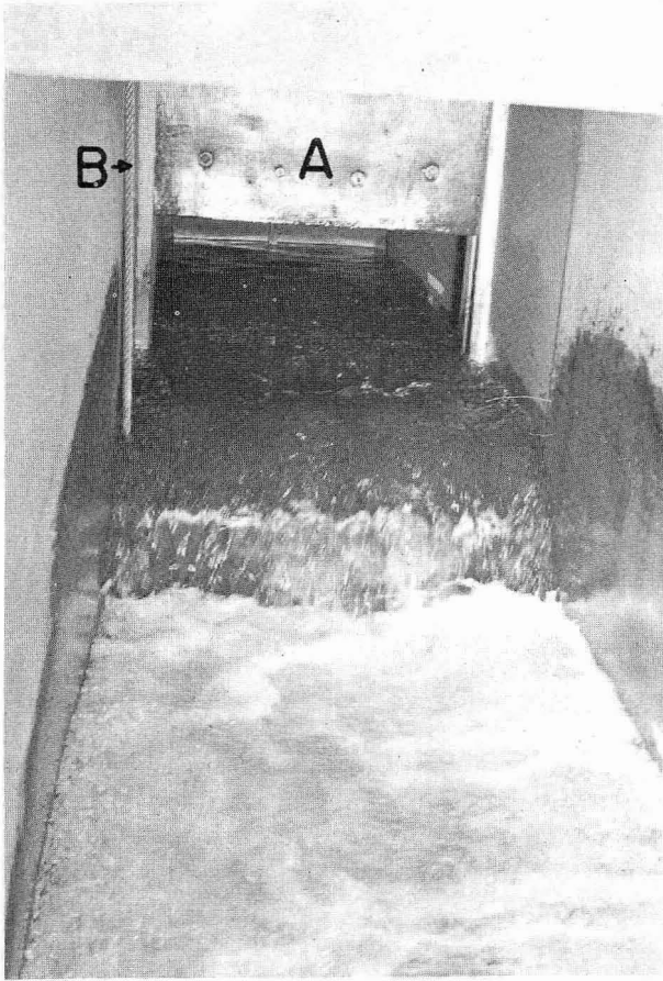
FIGURE 10.—Looking upstream from pool 66 over diffusion chamber and into lock. As fish enters lock, the drop gate (A) is lowered to isolate fish in lock. A motor-driven winch connected to the cable (B) raises a gate at base of lock, discharging water to elevation 51'.
