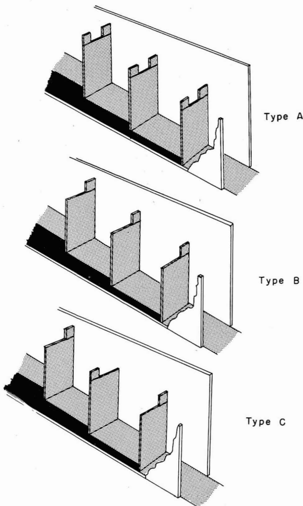
FIGURE 14.—Baffle placements showing notched, in-line, and alternate arrangements on weirs of 1-on-8-slope fishway.
