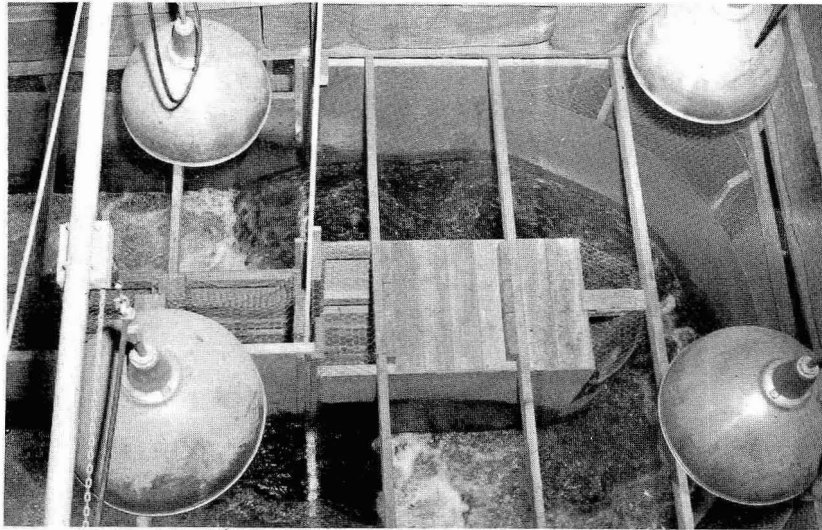
FIGURE 8.—Upper turn pool in the 1-on-8-slope fishway.
