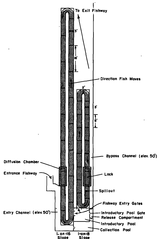
FIGURE 1.—Plan view of the 1-on-16-slope and 1-on-8-slope endless fishways with auxiliary approach channels and pools.
