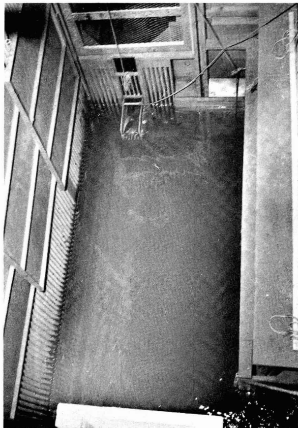
FIGURE 15.—Collection pool open for fish. Note finger fyke at entry gate (upper center).
