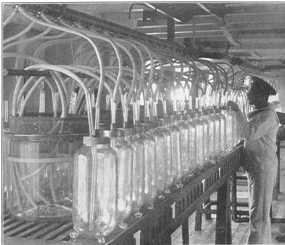
Main deck of steamer Fish Hawk, showing arrangement of McDonald automatic jars for hatching shad.
