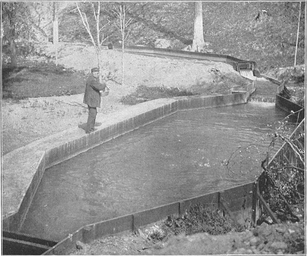
Artificial spawning pond and raceway, used in culture of rainbow trout at the Wytheville (Virginia) station.
