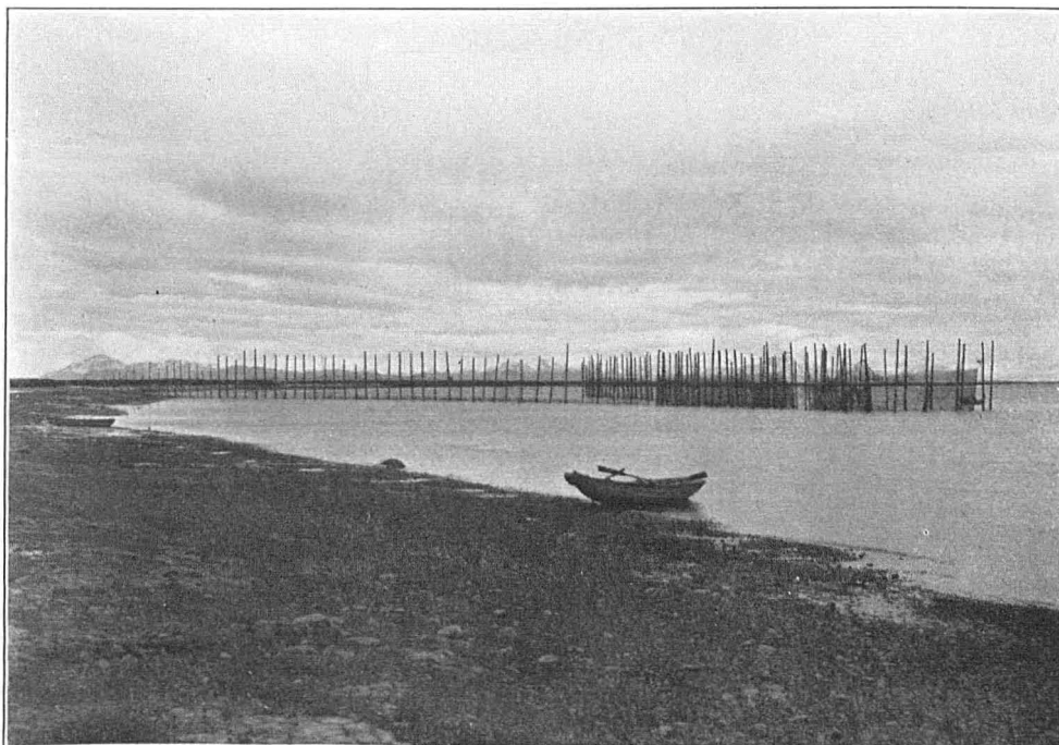
Salmon trap in an Alaskan river. This form of trap is extensively used in the Bristol Bay region, and takes immense quantities of salmon for the canneries. The largest traps have leaders more than half a mile long, and cost upward of $15,000.
