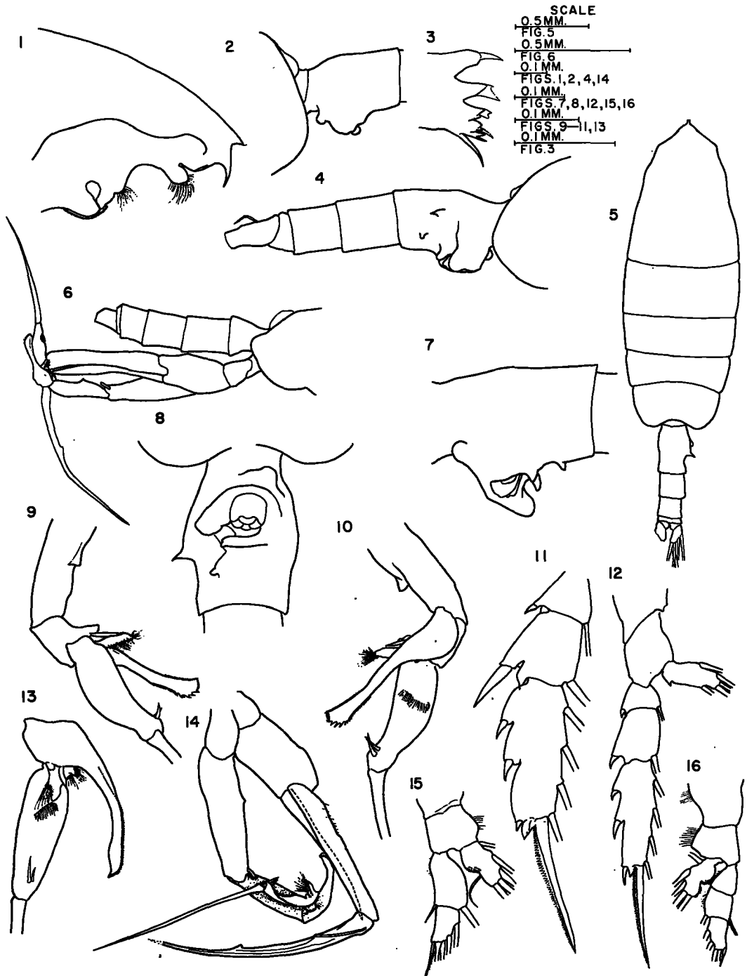
PLATE 2.— Euchaeta paraconcinna , new species. 1, female cephalon, lateral view; 2, female genital segment, lateral view; 3, female mandibular gnathal lobe; 4, female abdomen, lateral view; 5, female, dorsal view; 6, male abdomen, fifth legs, lateral view; 7, female genital segment, ventro-lateral view; 8, female genital segment, ventral view; 9, male left fifth leg, terminal segments, lateral view; 10, male left fifth leg, terminal segments, medial view; 11, female second leg, exopodite; 12, male second leg; 13, male left fifth leg, terminal segments, anterior view; 14, male fifth legs, posterior view; 15, female first leg; 16, male first leg. All figures drawn with aid of camera lucida; figure 4 of holotype, remaining figures of paratypes.
