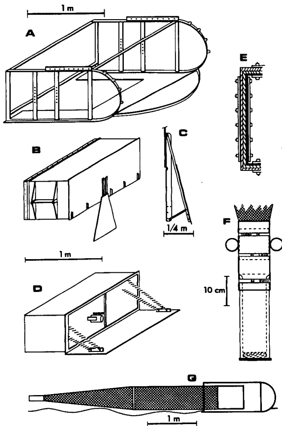
FIGURE 1.—Opening/closing epibenthic sampler: A) sled frame; B) box with door closed; C) detail, side view of shoe, hinge, and shoe adjustment device; D) box with door open showing flowmeter and springs for closing door; E) schematic net attachment, solid line is box wall, two cross hatched lines are collars of coarse mesh liner (inner) and plankton net (outer), open bars are stainless steel straps with bolts; F) safety collar insert with rings for cable attachment protruding through collar and PVC cod end with threaded teflon plug; G) schematic lateral view showing sled, box, net, and canvas chafing gear.
